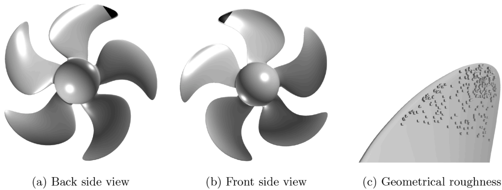
Fig. 3. (a) and (b): Roughness areas coloured black on the back side and front side of the refined blade; (c): zoomed view of the roughness elements inclusion.
