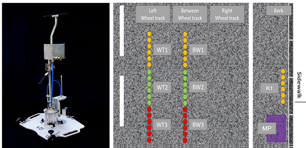
Fig. 2. left: WDS II (Photo Mats Gustafsson, VTI). On the right: Schematic figure over WDS sampling procedure for size distribution, road dust load and loss of ignition (WT = wheel track; BW = between the wheel track; K = adjacent to the kerb; MP = samples for microplastics adjacent to the kerb).
