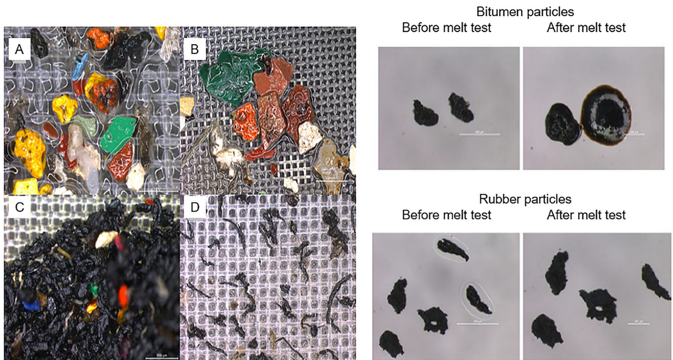
Fig. 4. to the left: Pictures A and B show paint particles from sweepsand. C shows rubber particles from sweepsand, and D shows rubber particles from washwater. Picture top right: bitumen particles before and after heating. Bottom picture: rubber particles before and after heating. Photos by Kerstin Magnusson, IVL Swedish Research Institute.
