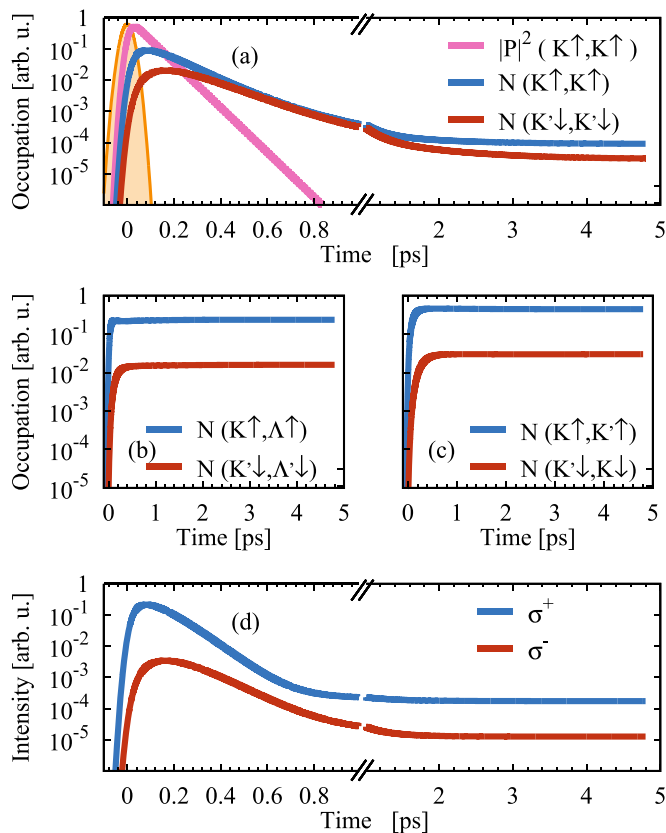
FIG. 3. Time evolution of exciton density and intensity of photoemission at 77K in WSe 2 . (a) shows the time evolution of the K\uparrow, K\uparrow and K'\downarrow, K'\downarrow exciton densities (note the log scale), (b) illustrates the corresponding K\uparrow, \Lambda\uparrow and K'\downarrow, \Lambda'\downarrow exciton densities, and (c) illustrates the K\uparrow, K'\uparrow and K'\downarrow, K\downarrow exciton densities. In (d), we show the corresponding emission intensities of \sigma^+ and \sigma^- light.
