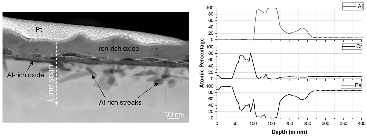
Figure 34: STEM-HAADF image (left) and EDX-data from line scan (right) of an iron-oxide-covered grain on FeCrAlSi after exposure to 5% O 2 + N 2 (bal.) at 600 °C for 168 hours
