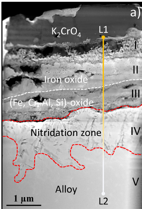
Figure 65: a) STEM-HAADF image (of TEM lamella) of Fe20CrAlSi after exposure to 5% O 2 + 20% H 2 O + N 2 (bal.) in the presence of KCl at 600 °C for 48 hours. The line L1 to L2 in a) corresponds to the STEM-EDX line-scan presented in b).
