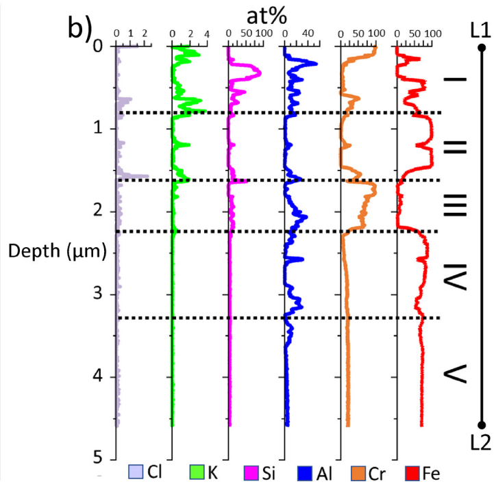
Figure 65: a) STEM-HAADF image (of TEM lamella) of Fe20CrAlSi after exposure to 5% O 2 + 20% H 2 O + N 2 (bal.) in the presence of KCl at 600 °C for 48 hours. The line L1 to L2 in a) corresponds to the STEM-EDX line-scan presented in b).
