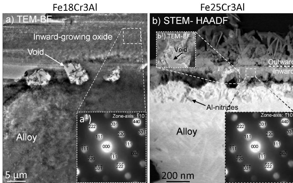
Figure 63: a) TEM-BF image of Fe18Cr3Al and b) STEM-HAADF of Fe25Cr3Al after exposure to 5% O 2 + N 2 (bal.) in the presence of K 2 CO 3 at 600 °C for 48 hours. a 1 ) and b 2 ) shows the CBED patterns in the inward-growing oxide of the respective alloys.
