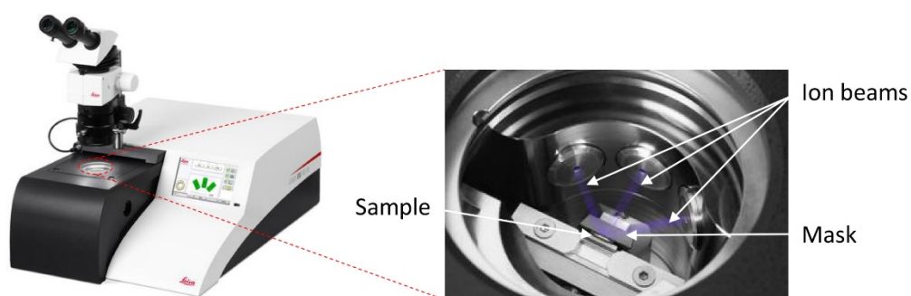
Figure 22: Picture of the BIB instrument used in this study (left). The picture to the right shows a sample attached to a sample holder hat has been placed on the instrument stage. Three ion guns are directed toward the sample, which is covered by a mask.
