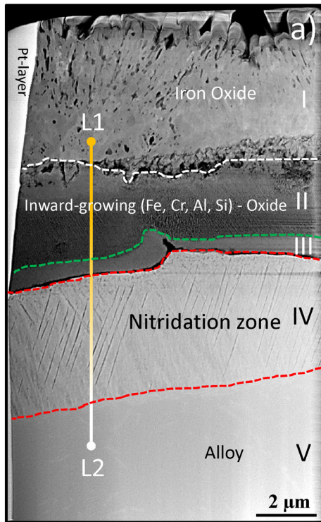
Figure 64: a) STEM-HAADF image (of TEM lamella) of Fe15CrAlSi after exposure to 5% O 2 + 20% H 2 O + N 2 (bal.) in the presence of KCl at 600 °C for 48 hours. The line L1 to L2 in a) corresponds to the STEM-EDX line-scan presented in b).
