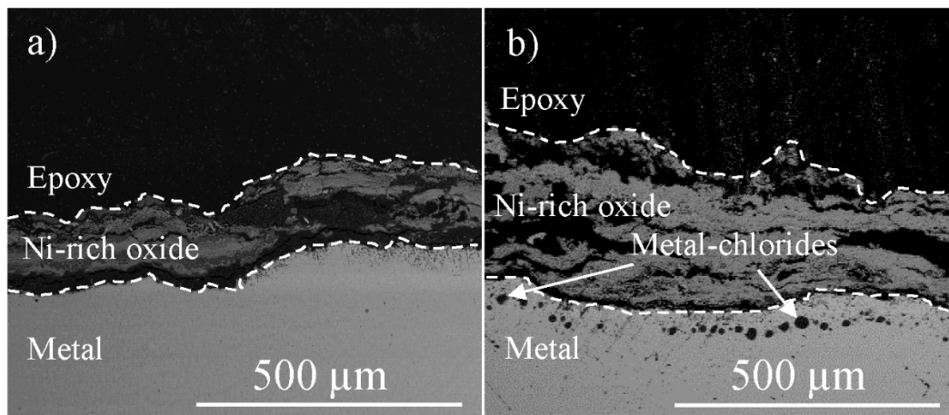
Figure 93: SEM-BSE cross-section images of the 16Mo3/IN625 sample ring on a) the leeward side and b) the windward side after exposure inside the waste-fired CHP boiler at a material temperature of 600 °C for 672 hours.
