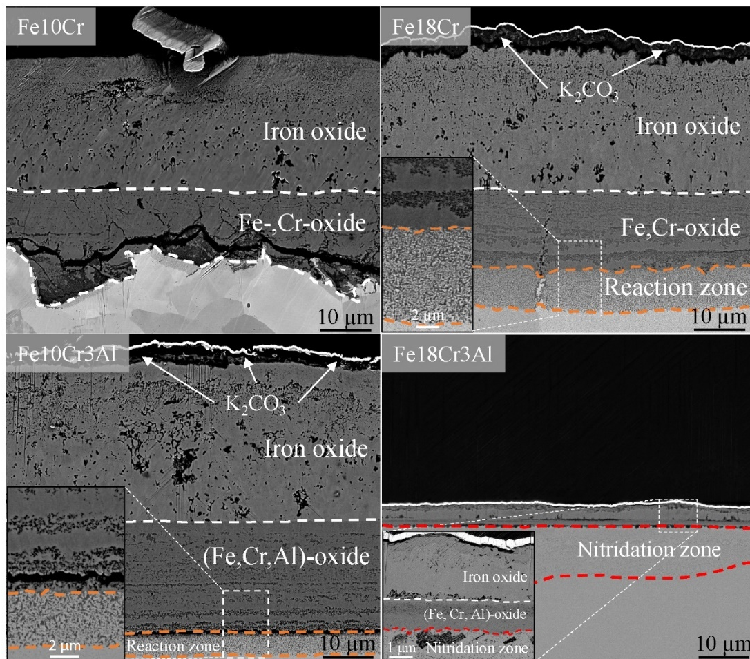
Figure 47: SEM-BSE cross section images of Fe10Cr, Fe18Cr, Fe10Cr3Al and Fe18Cr3Al after exposure to 5% O 2 + N 2 (bal.) in the presence of K 2 CO 3 at 600 °C for 48 hours.
