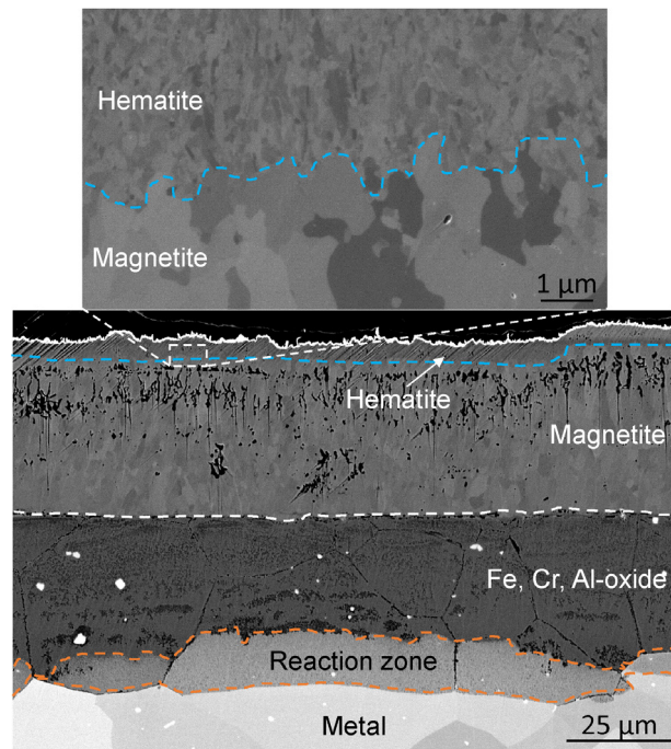
Figure 50: SEM-BSE cross section image of FeCrAl0Si after exposure to 5% O 2 + 20% H 2 O + N 2 (bal.) in the presence of KCl at 600 °C for 168 hours in a tube furnace.
