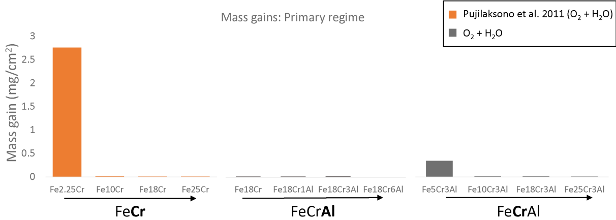
Figure 32: Average mass gains of FeCr(Al) model alloys after exposure to 5% O 2 + N 2 (bal.) at 600 °C for 24 hours.
