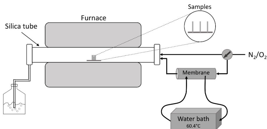
Figure 16: Schematic illustration of the tube furnace set-up used in this study.
