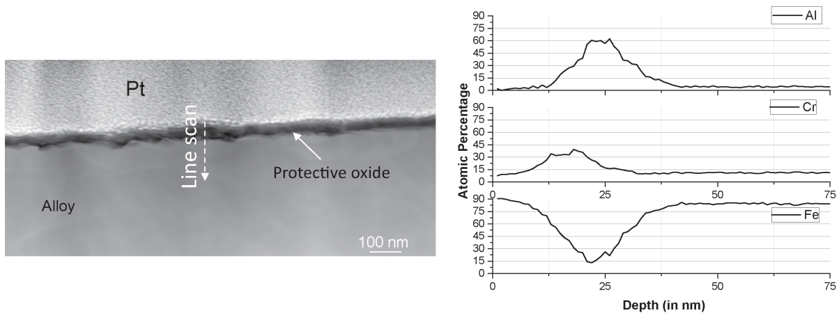
Figure 35: STEM-HAADF image (left) and EDX-data from line scan (right) of a protective grain on FeCrAlSi after exposure to 5% O 2 + N 2 (bal.) at 600 °C for 168 hours.
