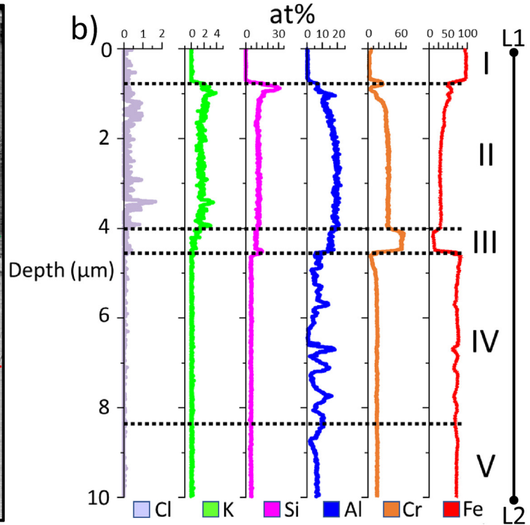
Figure 64: a) STEM-HAADF image (of TEM lamella) of Fe15CrAlSi after exposure to 5% O 2 + 20% H 2 O + N 2 (bal.) in the presence of KCl at 600 °C for 48 hours. The line L1 to L2 in a) corresponds to the STEM-EDX line-scan presented in b).
