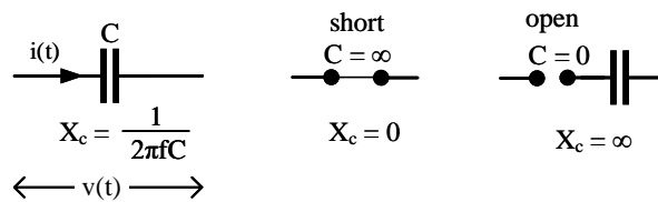
Fig. 1: Short circuit and open circuit of a capacitor.
