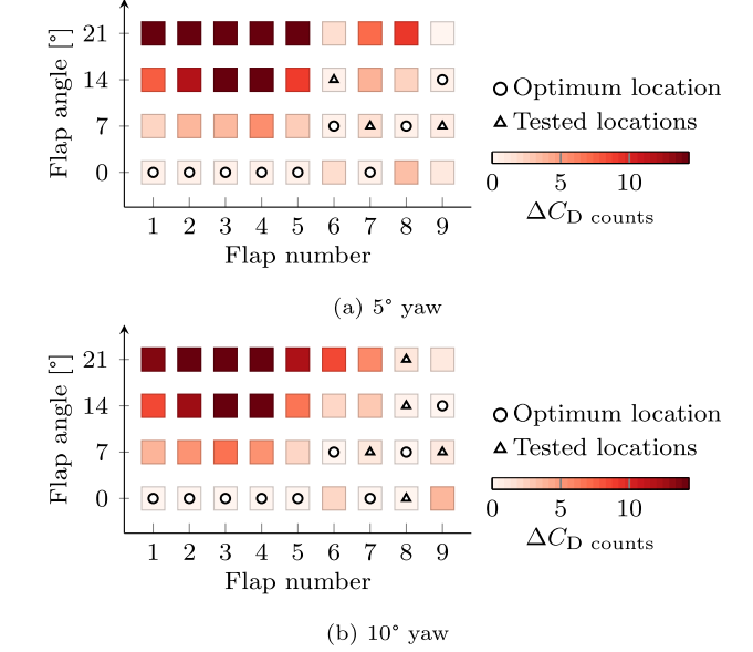
Fig. 21. Sensitivity to flap angle changes of each flap, while keeping the other flap angles constant at the best found design. Tested design locations only include designs which were explicitly tested.
