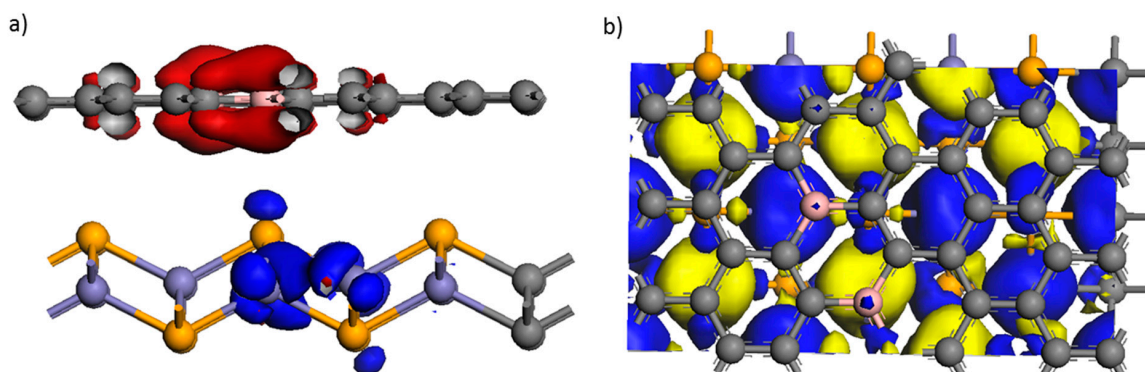
Figure 4. (a) Two states residing at E_F of \alpha -spin character, hole state (blue) of [\text{FeSe}]^h_{\text{AFM}} , and electron state (red) of [\text{B}\backslash=/\text{B}]^e . (b) resulting spin density of [\text{FeSe}]^h-[\text{B}\backslash=/\text{B}]^e . Magnetic structure is seen to change (compare Figure 3) reflecting the [\text{FeSe}]^h_{\text{AFM}} , while spurious spin on the boron doped graphene manifests the [\text{B}\backslash=/\text{B}]^e electron doping of this subsystem.
