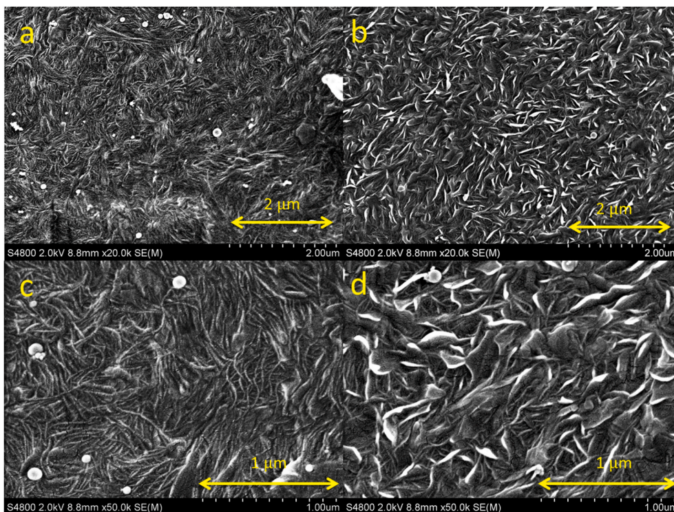
Fig. 3. SEM images of permanganate-etched 3 wt% C 8 -Al 2 O 3 nanocomposites with 0 wt% HDPE (left) and 4 wt% HDPE (right).
