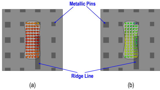
Fig. 8. Illustrations for field-distributions: (a) E-field. (b) H-field.
