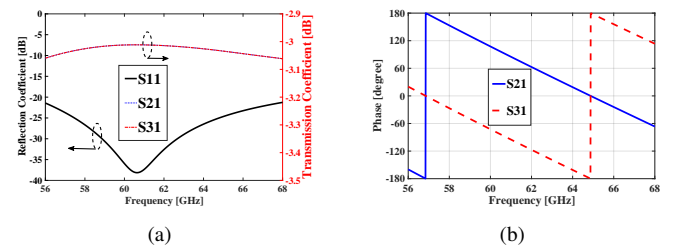
Fig. 15. Simulated S-parameter results of designed hybrid transition from WR-15 to RGW. (a) Amplitude. (b) Phase.
