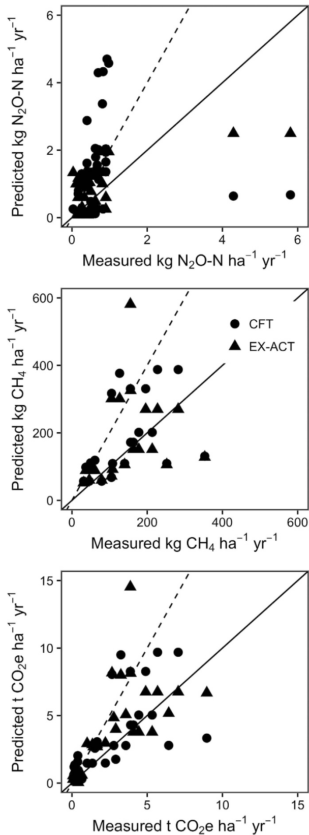
Figure 1. Comparison between measured and calculator-predicted soil fluxes for N 2 O, CH 4 , and the net balance (CO 2 e). The solid line is a 1:1 line; data points above this line represent an over-estimation of GHG emissions by the calculator. The dashed line is a 1:2 line; data points above this line represent an overestimation by a factor of 2 or more.
