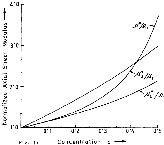
Fig. 1: Concentration c → The figure indicates that \mu^* is closer to the lower bound for values of c up to 0.35; thereafter, it is closer to the upper bound.
