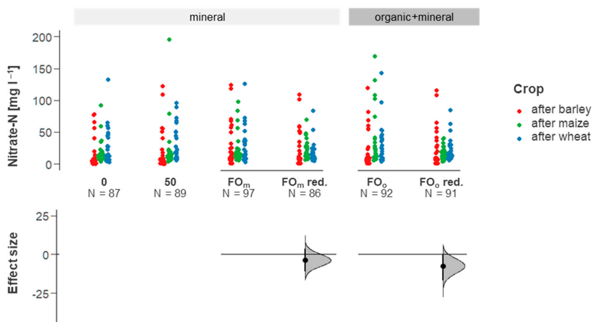
Figure 4. Estimation plot and effect sizes for \text{NO}_3\text{-N} concentrations under different fertiliser treatments and direct comparisons between fertiliser ordinance recommended (FO) vs. reduced (FO red.) fertilisation by fertiliser type (m: only mineral, o: combined organic + mineral) for all experimental seasons (N: sample size).
