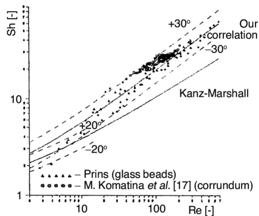
Figure 3. Mass transfer between coal particles and fluidized bed
