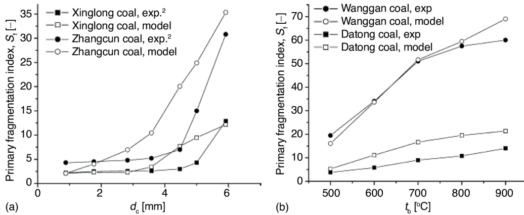
Figure 6. Primary fragmentation index, comparison with experimental results, influence of size of coal (a), influence of FB temperature (b)
