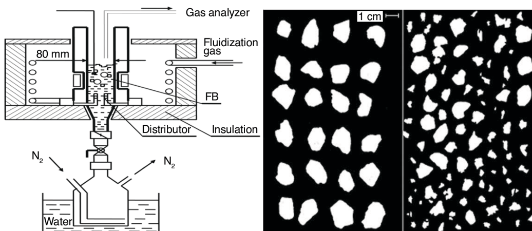
Figure 4. Experimental set-up & typical photograph of coal samples before/after devolatilization
