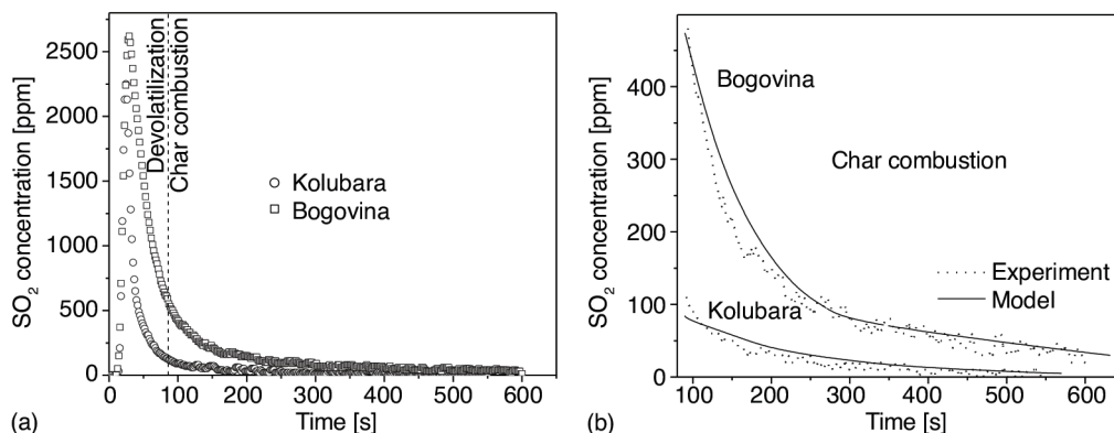
Figure 9. The \text{SO}_2 concentration at top of the bed during batch combustion of coal, T_{\text{bed}} = 750^\circ\text{C} , R_{\text{ch}} = 2\text{-}3.5\text{ mm} ; (a) experimental values during the whole process of combustion, (b) experimental values and model predictions during char combustion [54].
