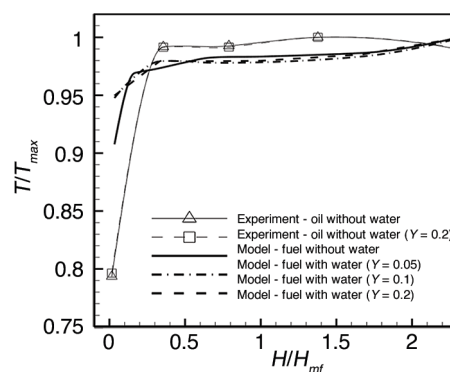
Figure 11. Normalized temperature profiles along fluidized combustor height.
