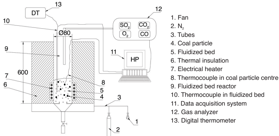
Figure 1. Experimental fluidized bed reactor, internal diameter 80 mm
