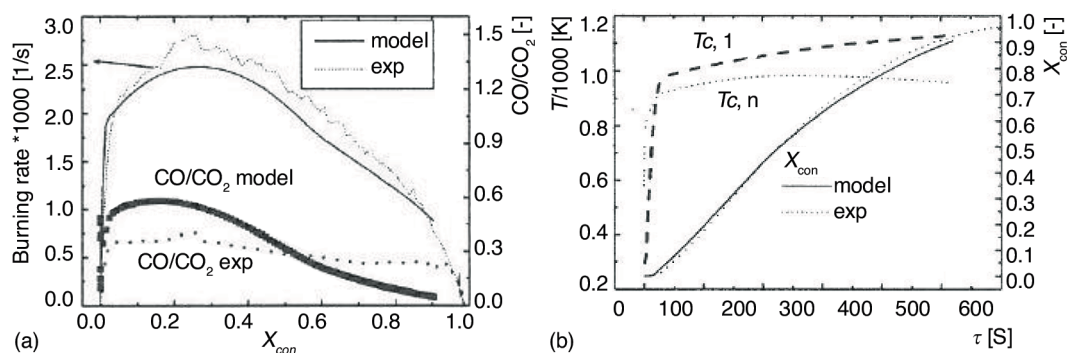
Figure 7. Experimental results and model predictions for 5 mm brown coal Aleksinac at 600 °C, (a) burning rate and CO/CO 2 ratio, (b) char particle temperature and carbon conversion degree vs. time
