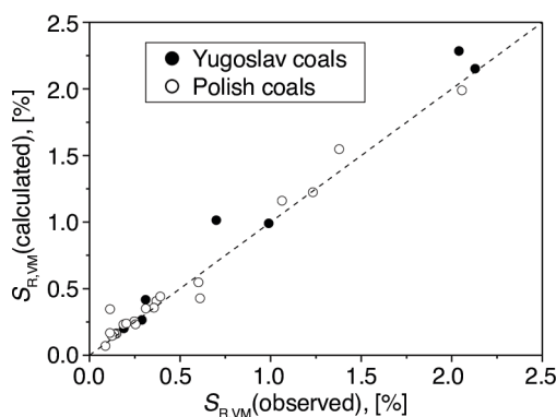
Figure 8. Experimental and calculated amount of released sulfur during devolatilization (% dry coal basis), for Yugoslav (●) and Polish (O) coals, [53]
