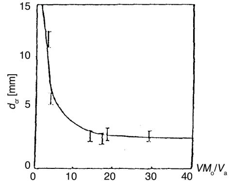
Figure 5. Critical fragmentation particle diameter for different coals [27]
