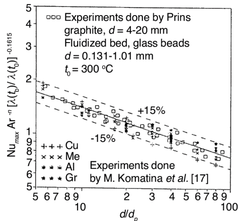
Figure 2. Heat transfer coefficient between coal particle and fluidized bed
