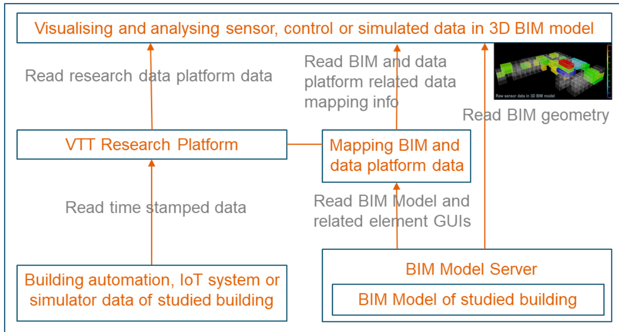
Figure 23. Solution for mapping, visualising and analysing Smart Otaniemi data by 3D BIM Models via VTT research platform.
