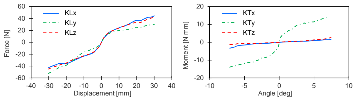
Figure 6. Stiffness splines.
