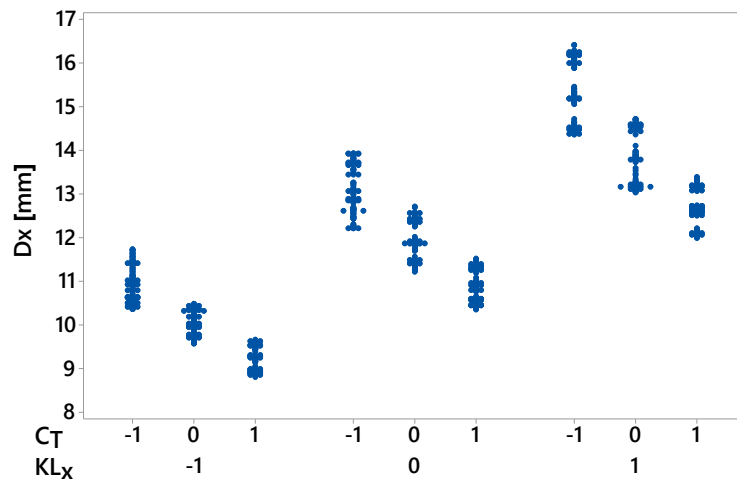
Figure 13. Maximum displacement in the x -direction with counter load.
