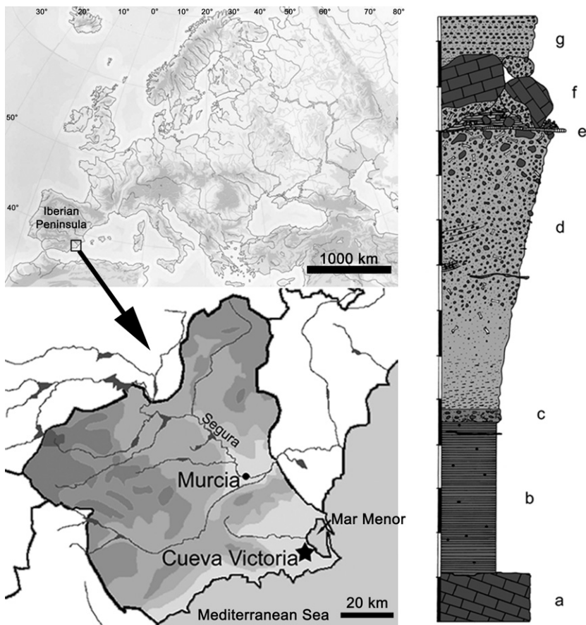
FIGURE 1 | Geographical location and simplified stratigraphy (redrawn from Ferrández et al., 1989; Gibert et al., 1992b, 1999, 2006) of Cueva Victoria (Murcia, Spain). a: Triassic limestone and dolomite; b: red clays ( terra rosa ) laminated with manganese nodules; c: reworked clays and first exogenous sediments; d: fossiliferous breccia; e: calcite layers; f: material of the mining exploitation; g: recent sediments.
