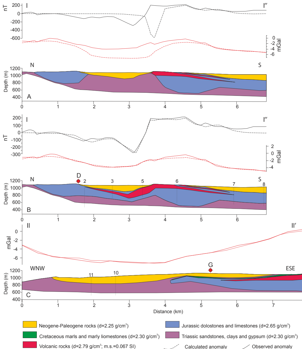
FIGURE 5. A–B) 2D integrated gravity and magnetic models of profile I–I’' and C) II–II’' gravity model. For the I–I’' profile, models A) without and B) with hydrogeological continuity are shown (d: density; m.s.: magnetic susceptibility). Numbers along the profiles represent TEM soundings; capital letters mark wells position as in Figure 1.
