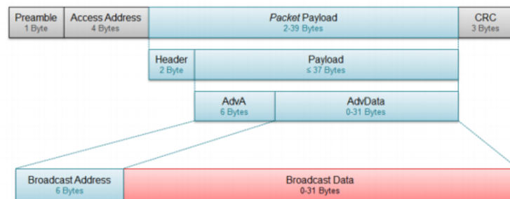
Figura 2.4: BLE broadcast packet[2]
