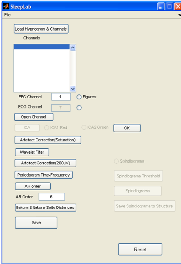
Fig. 6. A screen-shot of the user interface. The Save button exports all the results and models for comparison and statistical studies.
