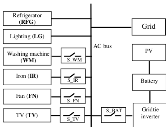
Figure 1. Architecture of proposed system – Electrical part.
