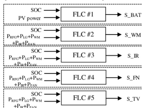
Figure 2. Architecture of proposed FLC.
