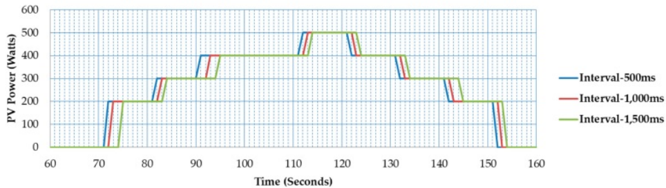
Figure 8. PV power simulated on a 10-s basis.
