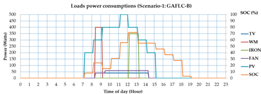
Figure 20. Power consumption of GAFLC-B in Scenario 1.
