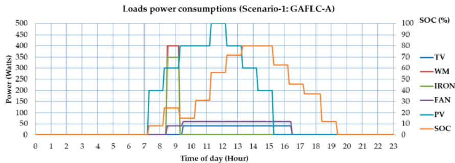
Figure 19. Power consumption of GAFLC-A in Scenario 1.
