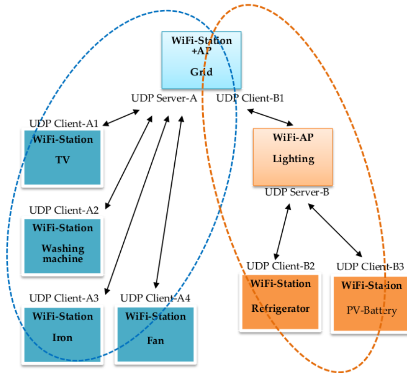
Figure 5. WiFi configuration.
