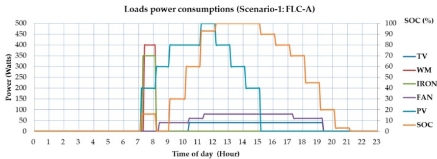
Figure 17. Power consumption of FLC-A in Scenario 1.
