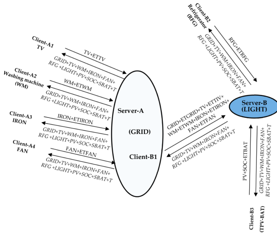
Figure 6. Data communication protocol.
