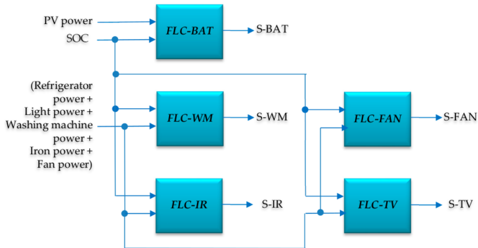
Figure 2. The architecture of the proposed FLC.
