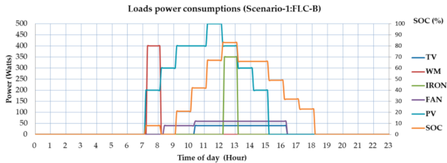
Figure 18. Power consumption of FLC-B in Scenario 1.
