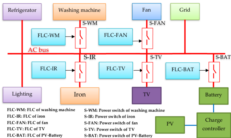
Figure 1. The architecture of electrical system.
