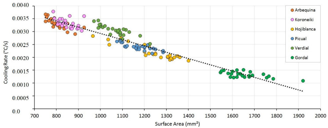
Figure 5. Correlation between surface area (mm) and cooling rate (°C/s) of different olive cultivars ( n = 150 ).
