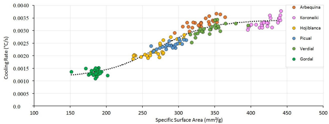
Figure 6. Correlation between specific surface area (mm 2 /g) and cooling rate (°C/s) of different olive cultivars ( n = 150 ).
