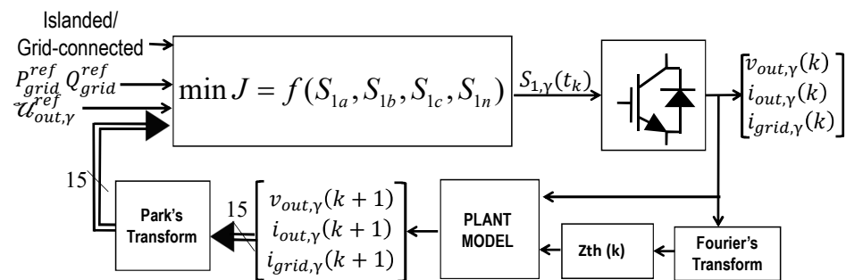
Figure 2. Block diagram.
