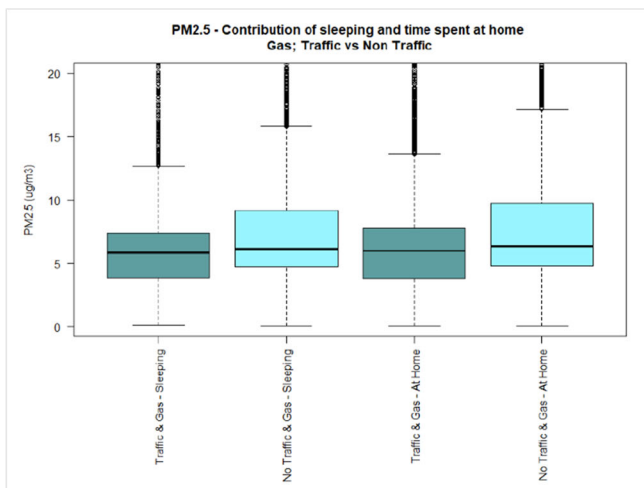
Fig. 6 \text{PM}_{2.5} personal exposure concentrations (5-min time average) during sleeping, and time spent at home, in houses located either near (dark colour) or away (light colour) from busy roads, using either gas (cadet
