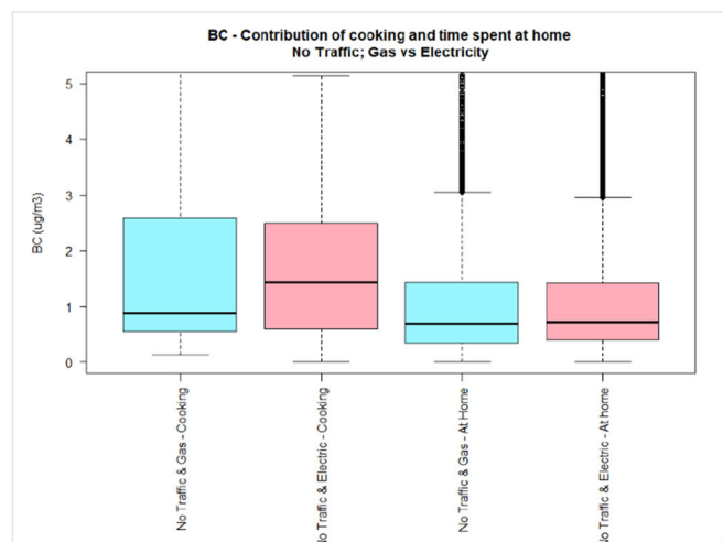
blue/light blue) or electric (dark pink/light pink) stove. The pollutant measurement distributions are non-normal (see main text) and axis are truncated. Full axis boxplots can be found in Fig. S2
