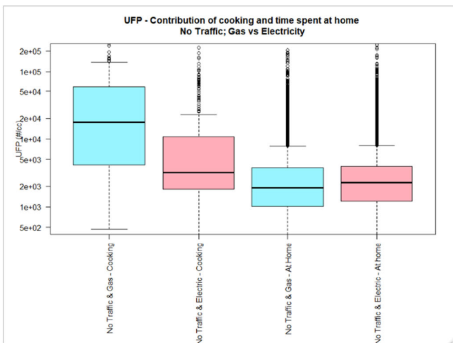
blue/light blue) or electric (dark pink/light pink) stove. The pollutant measurement distributions are non-normal (see main text) and axis are truncated. Full axis boxplots can be found in Fig. S1
