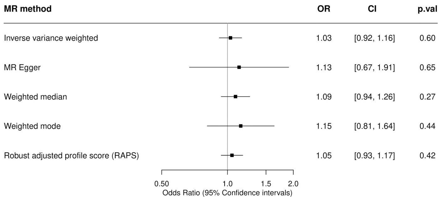
Fig 2. Two-sample MR estimates of the association between smoking initiation and the incidence of MS. A two-sample MR analysis was undertaken to obtain causal estimates of genetically predicted smoking initiation on MS susceptibility. MR and sensitivity analyses were performed using the TwoSampleMR R package with a comparison across 5 different methods. ORs are expressed per unit increase in log odds of ever smoking regularly (smoking initiation), with a 1 SD increase in genetically predicted smoking initiation corresponding to a 10% increased risk of smoking. The genetic variants used to proxy smoking initiation are the conditionally independent genome-wide significant SNPs taken from the GSCAN consortium detailed in Table A in S1 Data . The estimates of their association with MS are taken from the 2019 MS Chip IMISGC meta-analysis. CI, confidence interval; GSCAN, GWAS & Sequencing Consortium of Alcohol and Nicotine use; IMISGC, International Multiple Sclerosis Genetics Consortium; MR, Mendelian randomization; MS, multiple sclerosis; OR, odds ratio; p.val, p -value; RAPS, robust adjusted profile score; SD, standard deviation; SNP, single nucleotide polymorphism.
