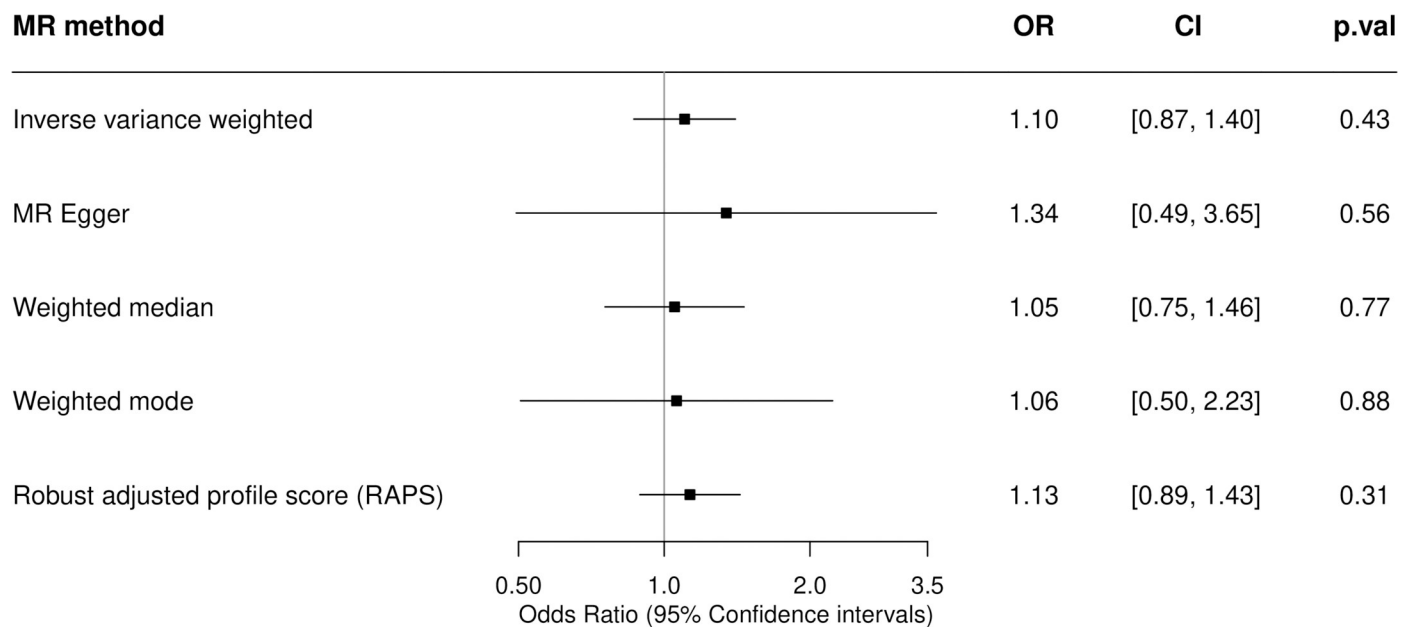
Fig 3. Two-sample MR estimates of the association between lifetime smoking and the incidence of MS. A two-sample MR analysis was undertaken to obtain causal estimates of genetically predicted lifetime smoking on MS susceptibility. MR and sensitivity analyses were performed using the TwoSampleMR R package with a comparison across 5 different methods. ORs are expressed per 1 SD increase of the lifetime smoking index. A SD increase in the lifetime smoking score is equivalent to an individual smoking 20 cigarettes a day for 15 years and stopping 17 years ago or an individual smoking 60 cigarettes a day for 13 years and stopping 22 years ago. The genetic variants used to proxy lifetime smoking are the independent genome-wide significant SNPs taken from the GWAS of lifetime smoking performed by Wootton and colleagues detailed in Table C in S1 Data . The estimates of their association with MS are taken from the 2019 MS Chip IMSGC meta-analysis. CI, confidence interval; GWAS, genome-wide association study; IMSGC, International Multiple Sclerosis Genetics Consortium; MR, Mendelian randomization; MS, multiple sclerosis; OR, odds ratio; p.val, p -value; RAPS, robust adjusted profile score; SD, standard deviation; SNP, single nucleotide polymorphism.
