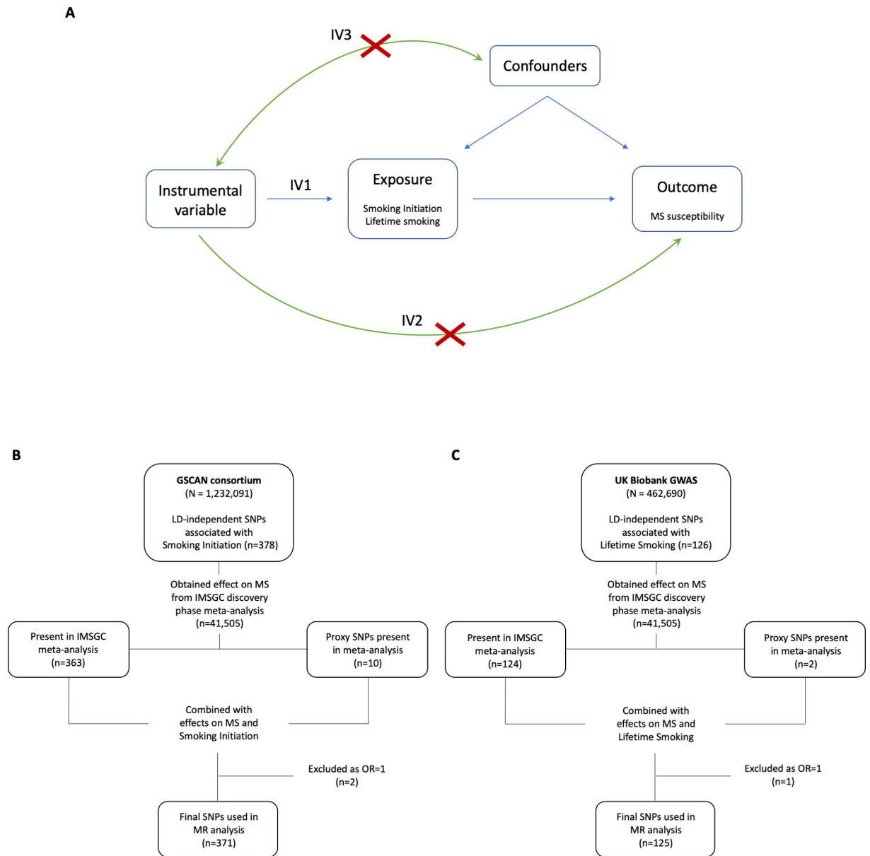
Fig 1. Schematic of MR analysis. (A) Directed acyclic graph of the MR framework investigating the causal relationship between smoking and MS. Instrumental variable assumptions: (1) the instruments must be associated with the exposure; (2) the instruments must influence MS only through smoking; and (3) the instruments must not associate with measured or unmeasured confounders in the smoking to MS relationship. (B and C) Flowchart for selection of genetic variants associated with smoking initiation (B) and lifetime smoking (C). GSCAN, GWAS & Sequencing Consortium of Alcohol and Nicotine use; GWAS, genome-wide association study; IMSGC, International Multiple Sclerosis Genetics Consortium; IV, instrumental variable; LD, linkage disequilibrium; MR, Mendelian randomization; MS, multiple sclerosis; OR, odds ratio; SNP, single nucleotide polymorphism.
