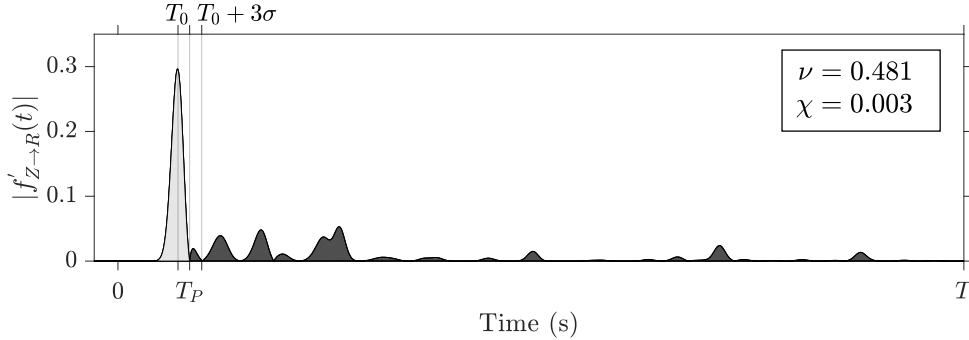
Figure 4. Illustration of our quality control metric, \nu , on a synthetic receiver function made in model IASP91 using AxiSEM. Synthetics were calculated for a M_w = 6.0 event, at 20 km depth. The receiver function shown corresponds to the recorded displacement 52^\circ away from our synthetic event. The metric weights the main P arrival relative to the P wave coda. The Gaussian width \tilde{\sigma} = 1.0 Hz, and the length of the window considered, T = 120 s. The light gray shaded area corresponds to the numerator in eq. (18).
