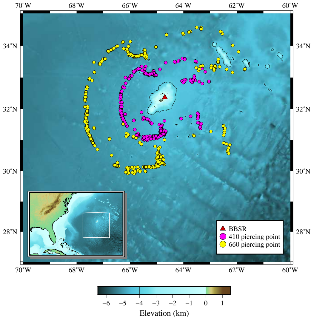
Figure 1. Bathymetry (Becker et al., 2009) of the study region, showing the location of Global Seismographic Network (GSN) station BBSR, and incoming P_{410s} and P_{660s} piercing points from the 226 earthquakes with high enough quality to be used in our receiver-function analysis. The bathymetric swell is roughly outlined by the 4 km depth contour. Note the absence of a well defined hotspot track, which would be expected to trend East-West.
