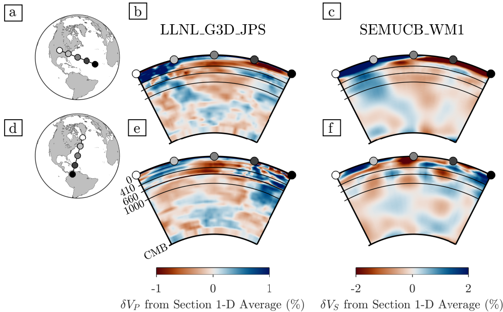
Figure 2. Cross sections centered on Bermuda through whole mantle tomography (b,e) V_P component of model LLNL_G3D_JPS (Simmons et al., 2015) and (c,f) V_S model SEMUCB_WM1 (French & Romanowicz, 2014). Wave speed perturbations are shown relative to the one-dimensional (1-D) average velocity profile for the region shown in the cross section. Note the consistently imaged low seismic velocity anomaly extending through the mantle transition zone, but not necessarily through the entire mantle, beneath Bermuda. The anomaly is particularly apparent in the North-South cross sections (e and f).
