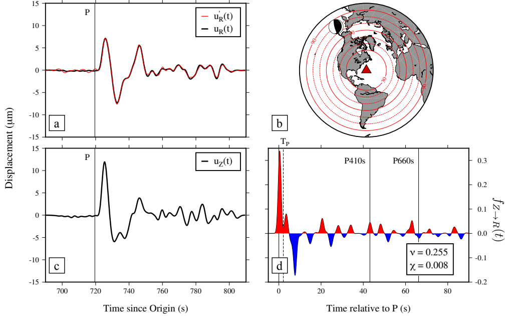
Figure 3. (a) Unfiltered radial and predicted radial ( u_R and u'_R ) and (c) vertical ( u_Z ) component displacement seismograms recorded in Bermuda for the June 14, 2005 M_W=6.8 earthquake at 53.9 km depth (C200506141710A). The vertical line shows the predicted P arrival time according to 1-D velocity model IASP91. (b) Map showing the event with its corresponding Global CMT focal mechanism (Ekström et al., 2012) solution. The red circles indicate different epicentral distances from BBSR. (d) Radial receiver function computed for this event using a Gaussian width factor \tilde{\sigma} = 1.0 Hz (see main text). The model quality factor, \nu , and data misfit, \chi , as discussed in the text, are included for reference.
