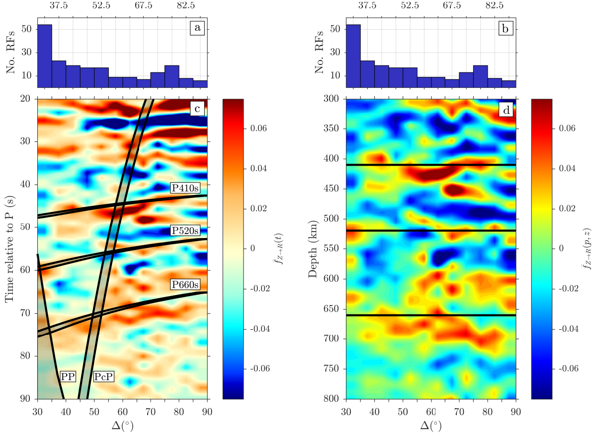
Figure 7. (a-b) Identical histograms showing the distribution with epicentral distance of the receiver functions that went into the construction of the panels below them. (c) Time-domain receiver functions arranged by epicentral distance. Binning is in 5^\circ increments starting at 30^\circ . Shaded gray regions indicate theoretical arrival times of PP , PcP , and relevant Pds phases from the mantle transition zone calculated using IASP91 according to eq. (20), for a range of earthquake depths between 0 and 653 km. Note the large signal from PP in the 30^\circ to 35^\circ bin, with a similar arrival time to P520s . (d) Depth-domain receiver functions, moveout-corrected using 1-D model IASP91. The 410 appears depressed, with a prominent signal between 50 and 80^\circ , but the resolution of the depth of the 660 is poor, as it appears to occur over a broader depth range.
