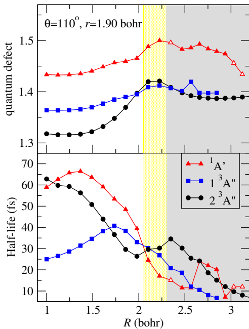
FIG. 8. Quantum defect and half-life along a cut of PES with fixed \theta = 110^\circ and r = 1.90 a_0 . The yellow area correspond to geometries where only the 1\ ^3A'' resonance is below the \tilde{B} threshold, while in the grey area the three resonances are below the \tilde{B} threshold. White-filled triangles correspond to the tentative fittings of hidden resonances (see Fig. 9).
