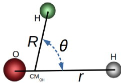
FIG. 4. Jacobi coordinates.
