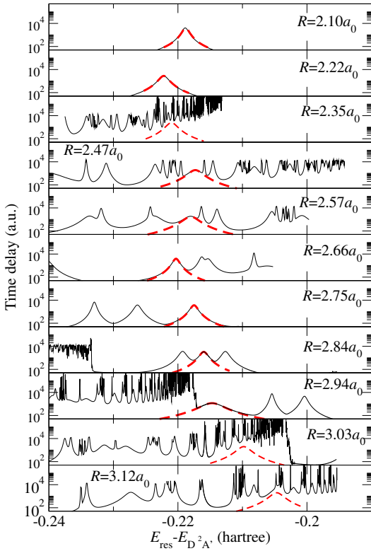
FIG. 9. Time delay for resonances of symmetry 1A' for the values of the R coordinate indicated. For each panel, the zero of energy is located at the energy of the \tilde{D} target state, so the resonances of the Rydberg series converging to \tilde{D} appear at approximately the same energy. Red-dashed lines are drawn using the parameters plotted in Fig. 8 for resonance 1A' , the thin red-dashed ones are only tentative resonances and are shown with white-filled triangles in Fig. 8.
