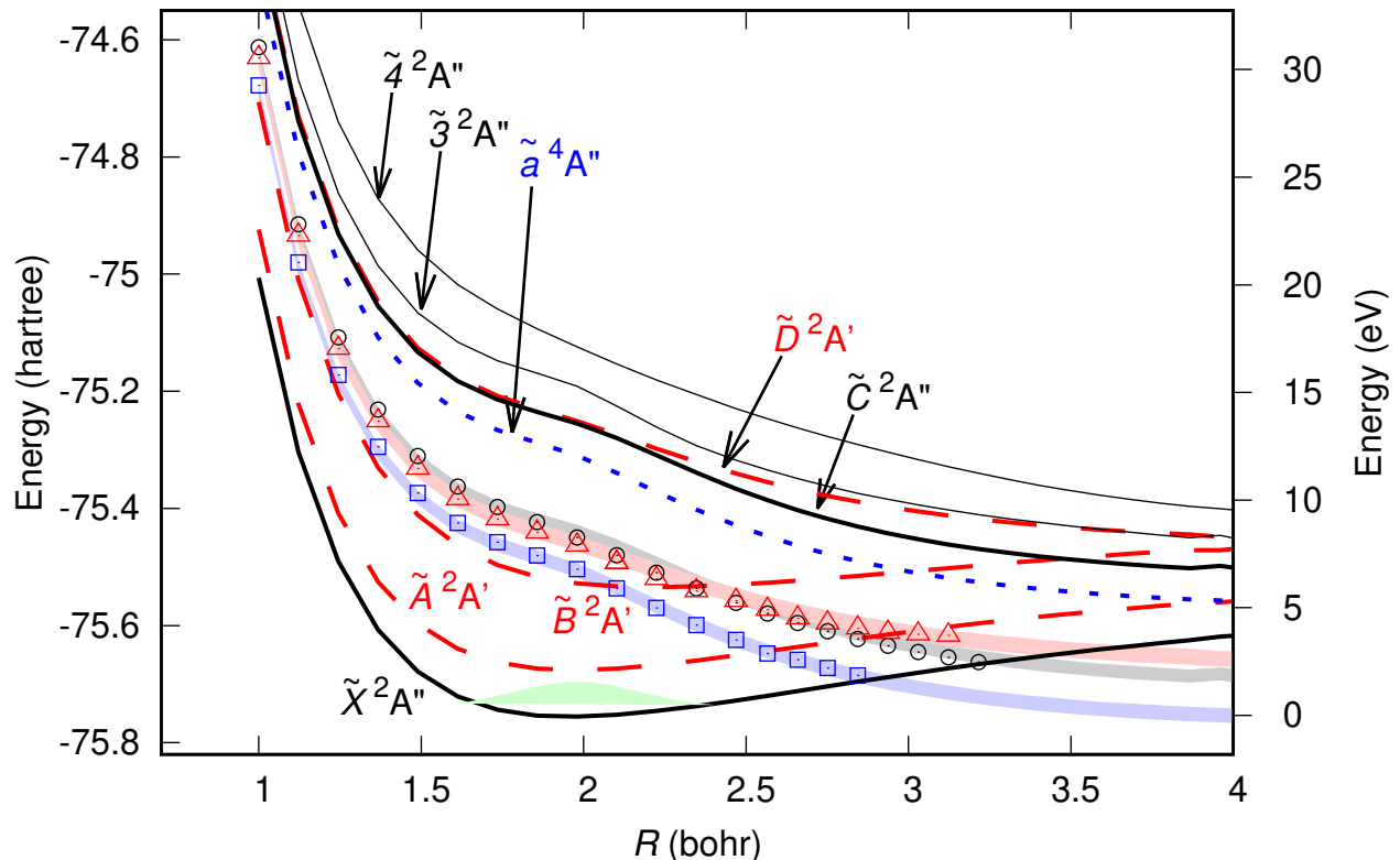
FIG. 5. Cut of the PESs along the Jacobi R -coordinate with \theta=110^\circ and r=1.90 a_0 . The lines correspond to the eight electronic states of \text{H}_2\text{O}^+ : {}^2A'' (solid black), {}^2A' (dashed red) and {}^4A'' (dotted blue). The blue squares ( 1\ {}^3A'' ), black circles ( 2\ {}^3A'' ) and red triangles ( 1\ A' ) correspond to the resonance positions obtained from RESON, when above state \tilde{B} , and the time delay method below. The blue stripe is obtained from the \tilde{a} state using quantum defect theory with 1.35 < \delta < 1.45 , the grey stripe is obtained from \tilde{C} with 1.3 < \delta < 1.4 , and red stripe is obtained from \tilde{D} with 1.4 < \delta < 1.5 . Target state labels are included for clarity. Also shown is the approximate ground state vibrational wavefunction (green shaded area at the bottom of the \tilde{X} state).
