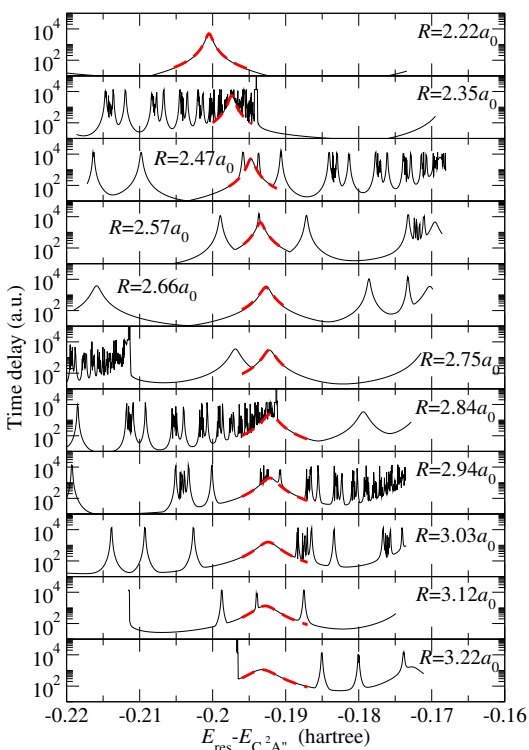
FIG. 11. Time delay for resonances of symmetry {}^3A'' . For each panel, the zero of energy is located at the energy of the \tilde{C} target state, so the resonances of the Rydberg series converging to \tilde{C} appear at approximately the same energy. Red-dashed lines are drawn using the parameters plotted in Fig. 8 for resonance 2\ {}^3A'' .
