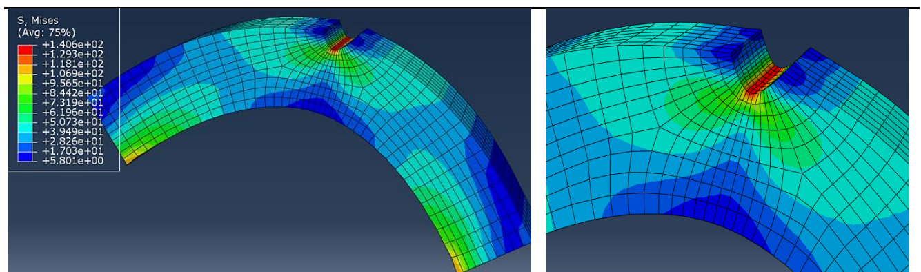
Figure 6. Distributions of Von Mises stress near the notch.
