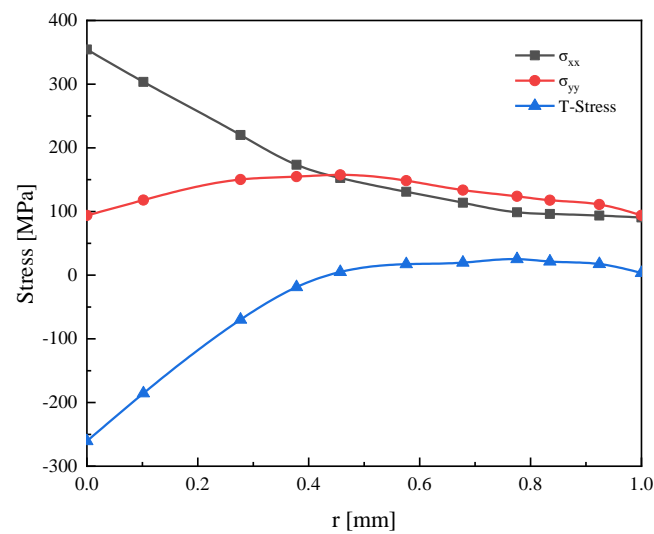
Figure 5. T-stress by stress different method.
