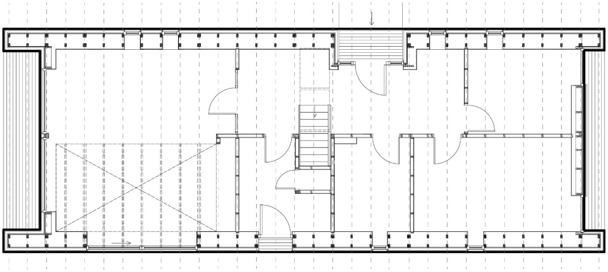
Ground Floor
