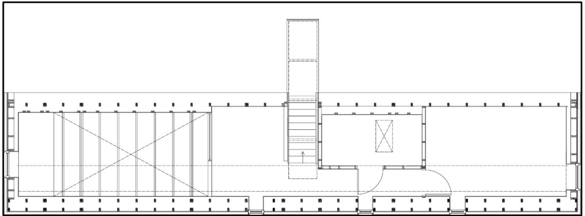
First Floor
