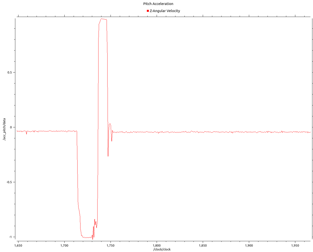
Figure 3.26: Acceleration on X axis (Pitch)
