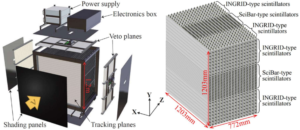
Fig. 5: Schematic view of the Proton Module (left) and its scintillator structure (right).
