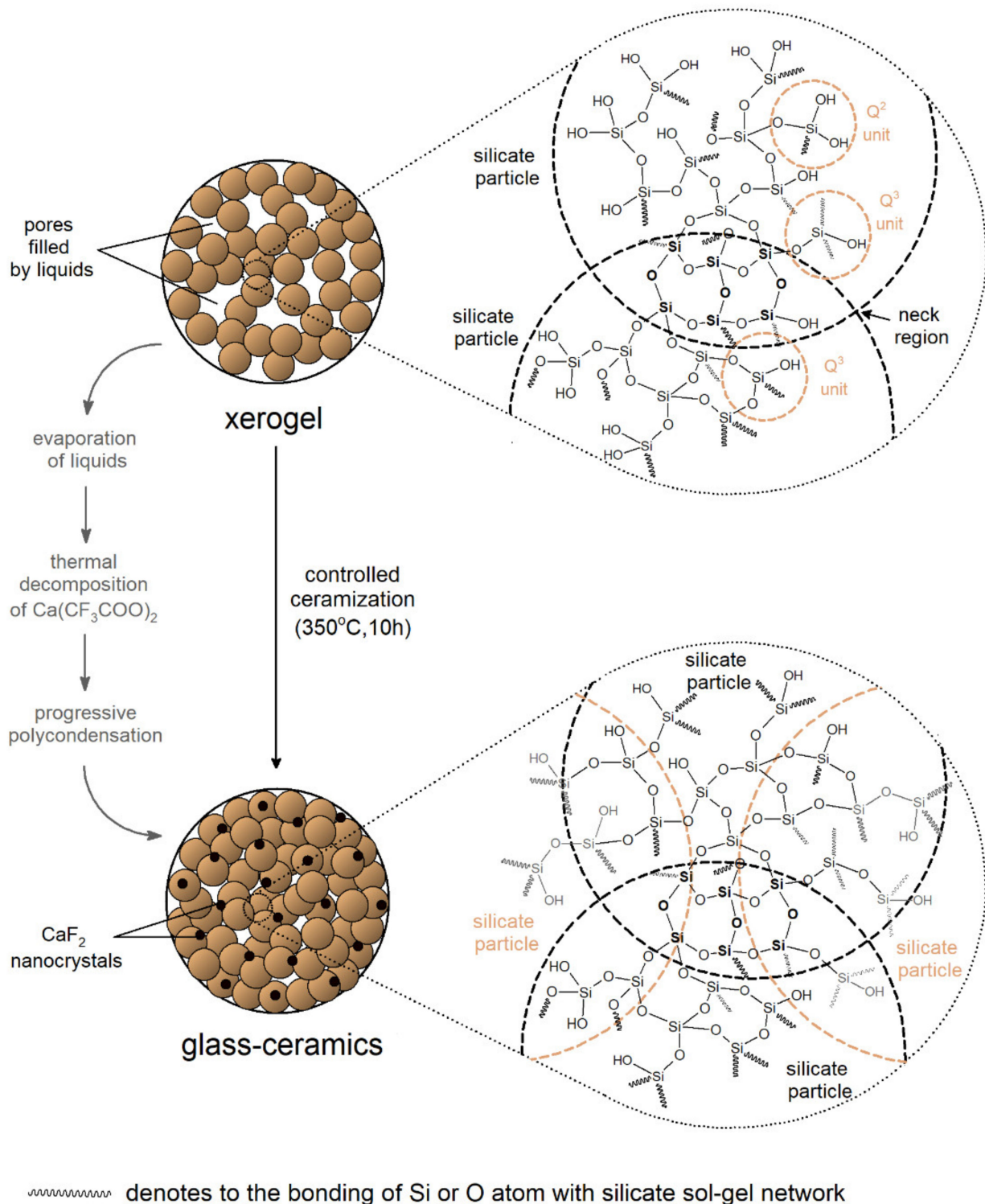
Figure 3. Graphical representation of structural transformation during controlled ceramization at 350^\circ\text{C} .
