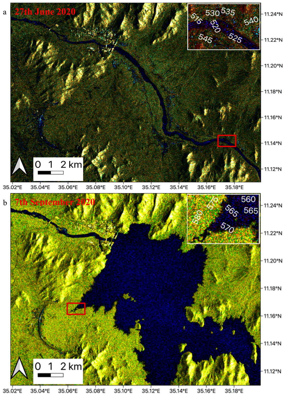
Figure 2. (a) Sentinel-1 for 27 June 2020 (prior to the filling process) and (b) 7 September 2020 (after the start of the filling process). The increased spatial extent of the reservoir can be observed in the second image on 7 September 2020. The inset figure shows the zoomed view of the region inside the red box to study the elevation contours inside the region. The contour values shown in the inset figure are in meters.
