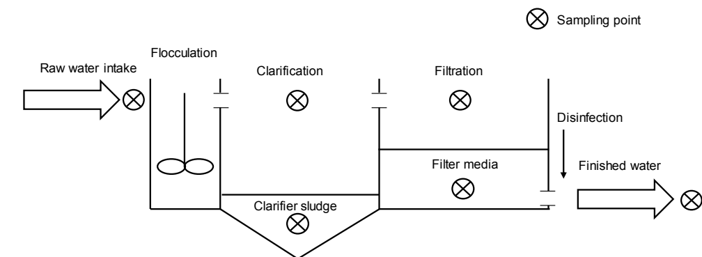
Figure 7. Schematic of a conventional treatment process and the sampling locations of this study.
