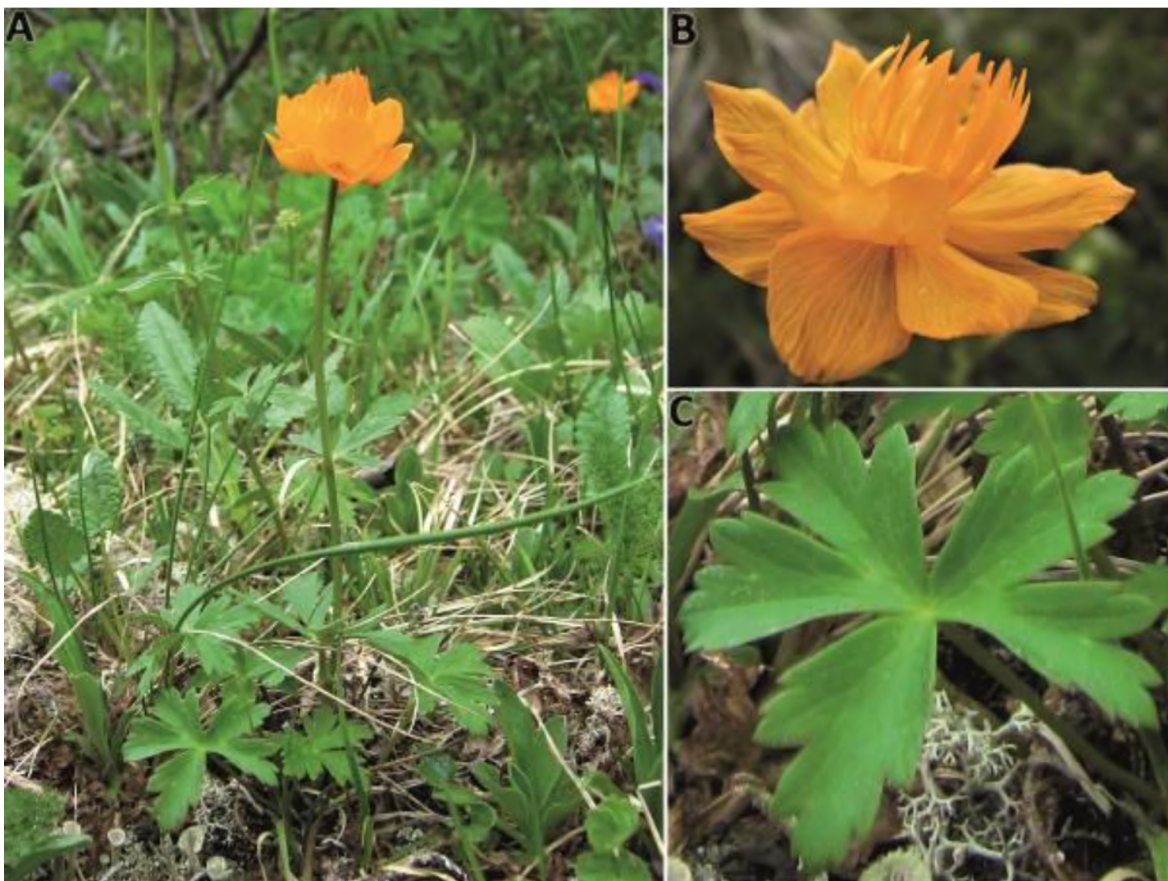
FIGURE 2. Photograph of Trollius austrosibiricus . A. Flowering plant; B. Flower; C. Leaf blade. (Photographs by E. Balde and A. Erst).
