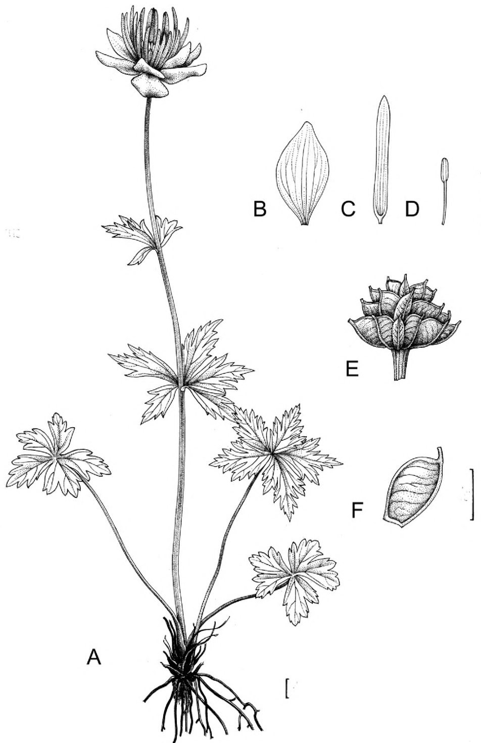
FIGURE 3. Trollius austrosibiricus . A – General view, B – Sepal, C – Petal, D – Stamen, E – Fruit, F – Follicle. Scale bar: 1 cm (A-F).
