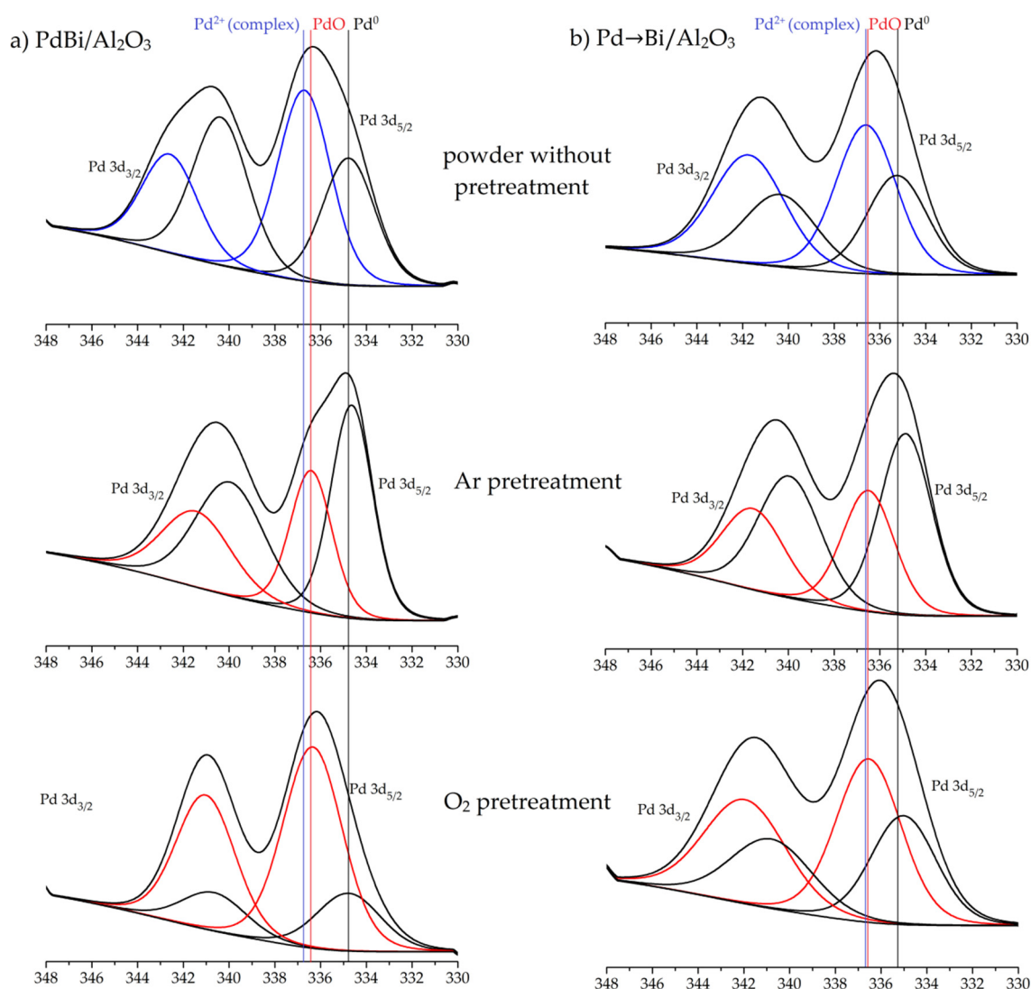
Figure 8. X-ray photoelectron spectra of the Pd 3d line of the catalyst surface after each stage of preparation (a) PdBi/ \text{Al}_2\text{O}_3 , (b) Pd \rightarrow Bi/ \text{Al}_2\text{O}_3 .
