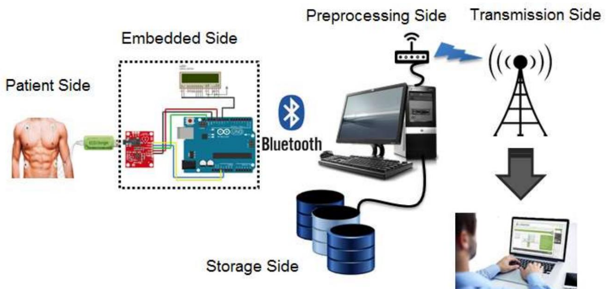
Figure 1. Overall ECG Signal Surveillance System Infrastructure
