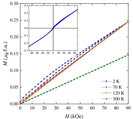
FIG. 4. Isothermal M versus H curves with an applied field 0 T \rightarrow 9 T \rightarrow 0 T recorded at 2, 70, 120 and 300 K. Insert: M versus H curve at 2 K to show the full symmetry.
