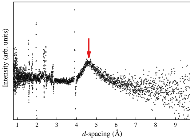
FIG. 8. Plot of the difference between NPD patterns at 95 and 120 K measured on the low resolution detector bank. A broad peak around 4.8 Å is marked by a red arrow, which corresponds to the (011)- and (110)-magnetic Bragg reflections and indicates short-range magnetic order appearing at 95 K.
