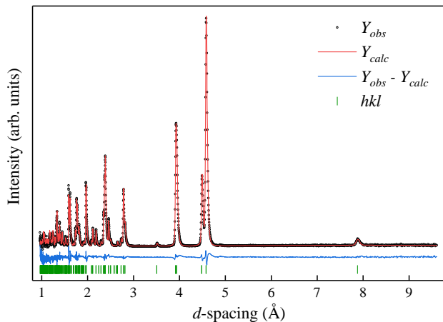
FIG. 5. Measured, calculated and difference curves from Rietveld refinement of the magnetic structure of \text{NaFeF}_3 at 2 K for the second detector bank of the WISH instrument at ISIS pulsed neutron and muon source (UK). The green ticks indicate reflections allowed by the magnetic symmetry (space group Pn'ma' ). The R_{wp} for this detector block is 3.70 %.
