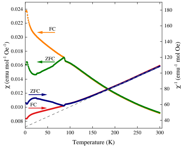
FIG. 2. Temperature dependency of the magnetic susceptibility \chi(T) at H = 10 kOe measured in ZFC-FC mode (left axis) and inverse magnetic susceptibility \chi^{-1} (right axis). The Curie-Weiss fit is shown as a dashed gray line.
