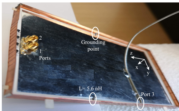
Fig. C.11: Antenna prototype.
