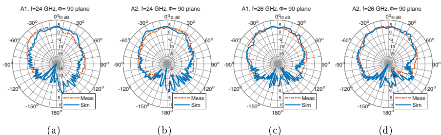
Fig. C.15: Radiation patterns of the two active antennas in the \Phi = 90^\circ at 24 and 26 GHz.
