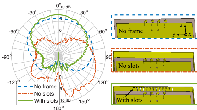
Fig. C.3: IEEE gain radiation pattern of the in-phase array combination at 26 GHz for the \Phi = 0^\circ cut.
