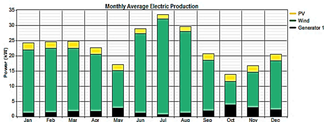
Figure 4. Contribution of the power units for 92% utilization of renewable resources.
