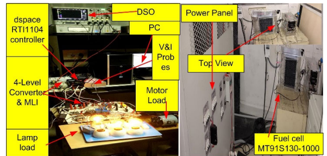
FIGURE 23. Experimental setup.
