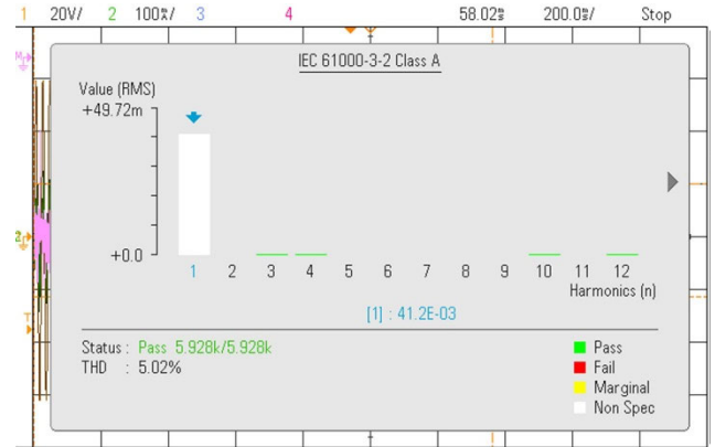
FIGURE 22. Experimental THD.
