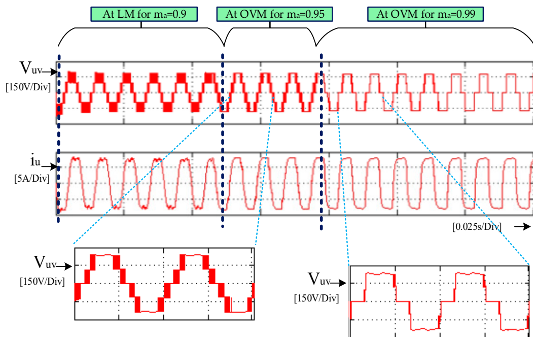
Figure 10. Simulation result for modulation range ( 0.9 < M_a \leq 0.99 ).
