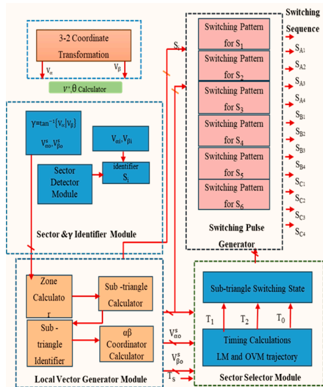
Figure 9. MLI SVM MATLAB-Simulink implementation flow chart.
