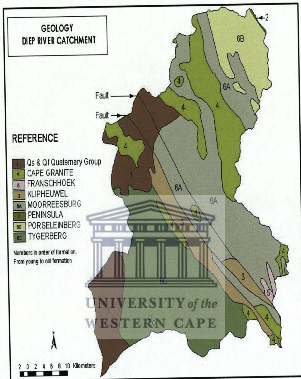
Figure 2.2 Geology of the Diep River Catchment (DWAf).
