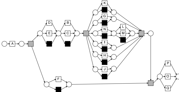
Fig. 6 Process model mined with the IMi: model \mathcal{I} (Petri net).
