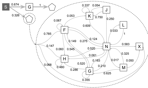
Fig. 14 HAT of cluster C_2 = C'_2 fixing \ell = 100
