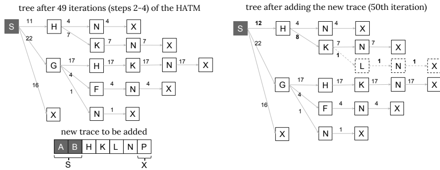
Fig. 11 The example shows how the new trace ABHKLNP is added to the tree by the HATM during the 50-th iteration: after converting the trace into SHKLN, it is added following the common initial path SHK (increasing the edge labels) and adding the new branch LNX.
