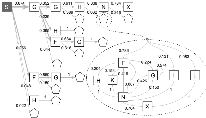
Fig. 13 HAT of cluster C_2 = C'_2 fixing \ell = 30
