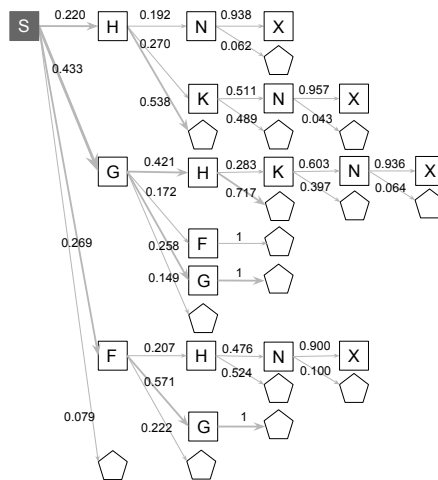
Fig. 15 HAT of cluster C_4 = C'_4 fixing \ell = 30
