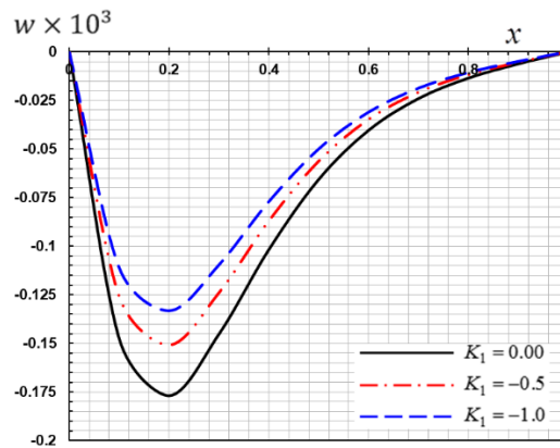
Fig. 2 Deflection w under the influence of variable thermal properties
