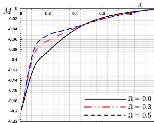
Fig. 9 Bending moment M vs angular velocity \Omega
