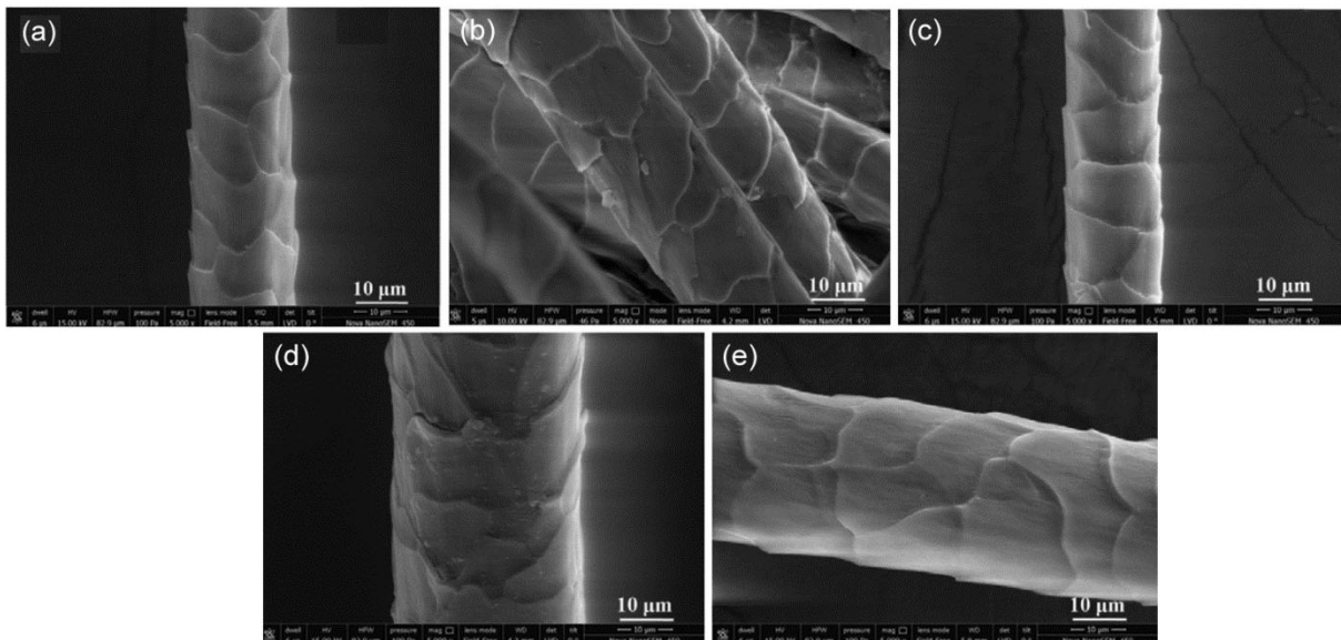
Fig. 2 — FE-SEM images of wool fibres (a) blank, (b) TG3, (c) LP2, (d) LC3, and (e) PR2
