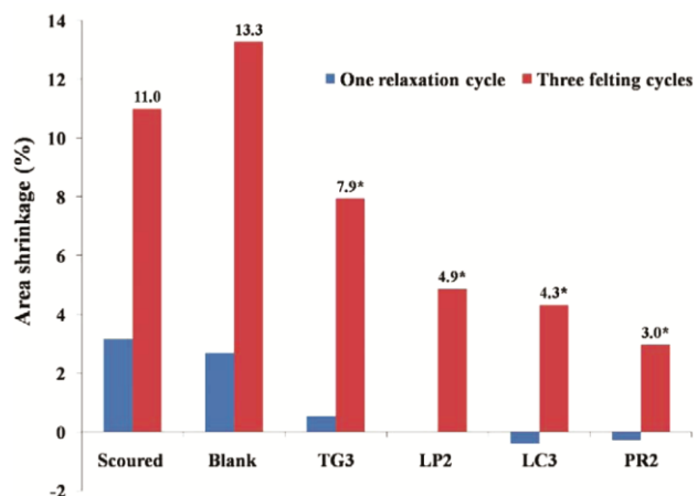
Fig. 4 — Effect of selected enzyme concentration on dimensional stability of wool fabrics (*significant at 5% level of significance)
