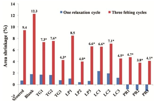
Fig. 1 — Area shrinkage of wool fabrics treated with transglutaminase, lipase, laccase, and protease enzymes in concentration range 0.5–2% (*significant at 5% level of significance)
