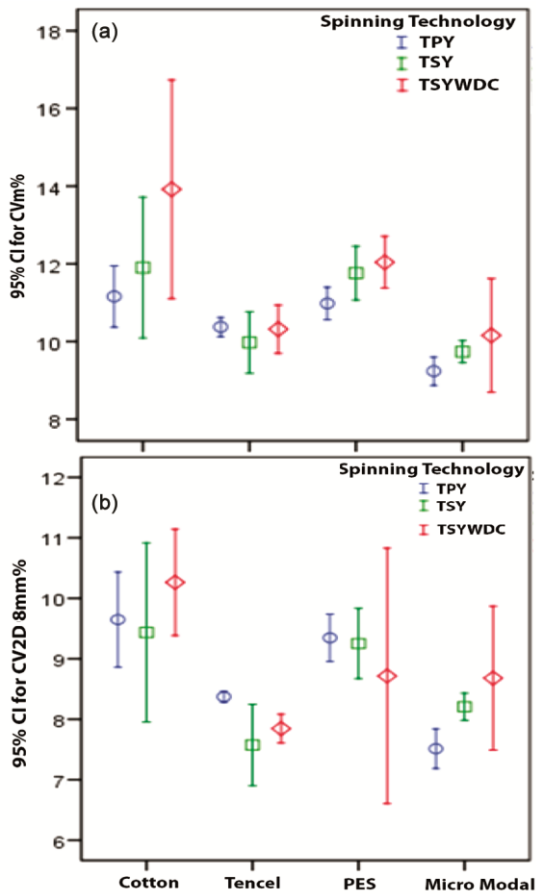
Fig. 4 — 95% confidence intervals for unevenness and optical unevenness values of TPY, TSY and TSYWDC
