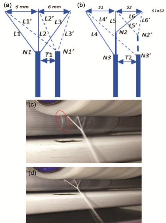
Fig. 5 — Changes in the geometry of spinning triangles during production for TSYWDC (a), and TSY (b), respectively (N= yarn formation point, L= strand length, S= strand space, T= displacement for yarn formation point), fibre loss caused from non-stationary spinning for TSYWDC (c), and two yarn formation points for TSY (d)
