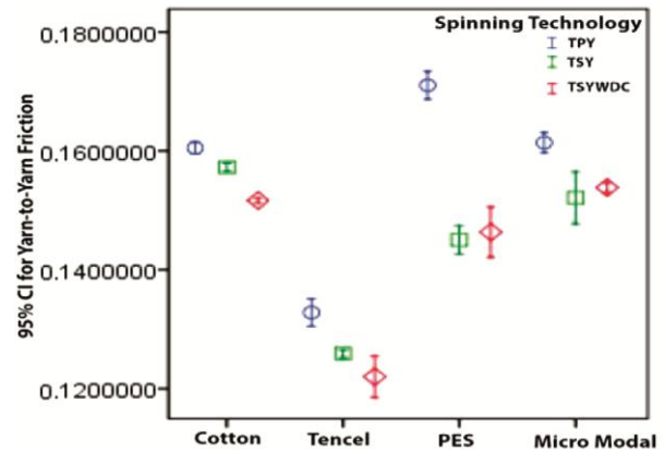
Fig. 6 — 95 % confidence interval graphs for yarn-to-yarn friction coefficients of TPY, TSY and TSYWDC
