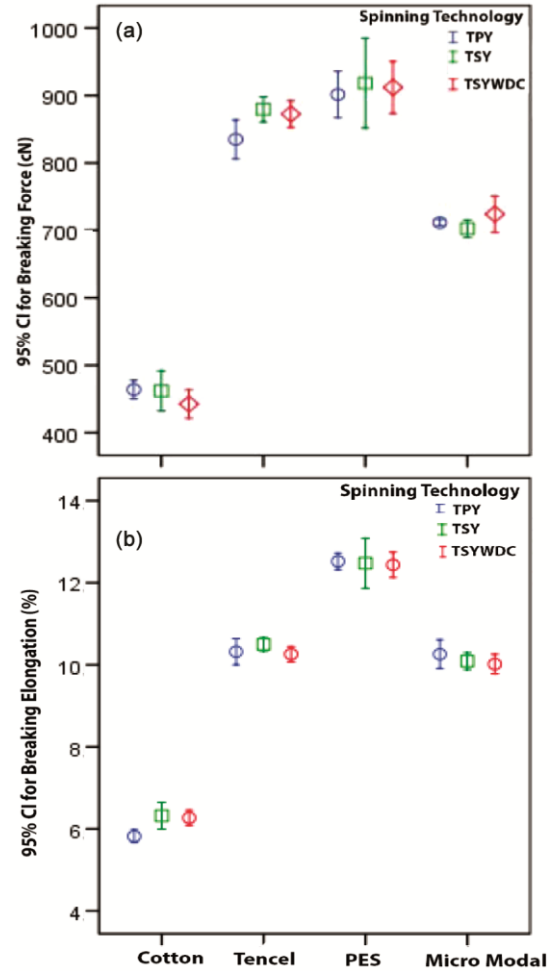
Fig. 3 — 95% confidence interval graphs for breaking force and breaking elongation of TPY, TSY and TSYWDC yarns
