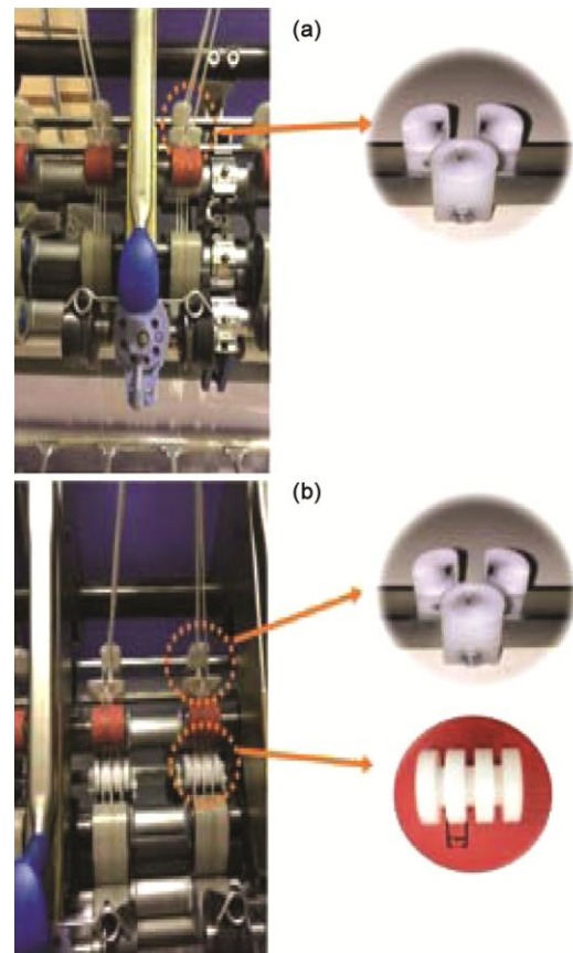
Fig. 1 — (a) Three-strand yarn – TSY and (b) three-strand yarn with delivery cylinder – TSYWDC
