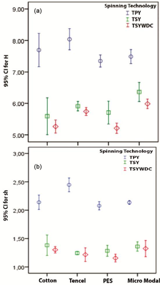
Fig. 2 — 95% confidence interval graphs for hairiness values of TPY, TSY, and TSYWDC
