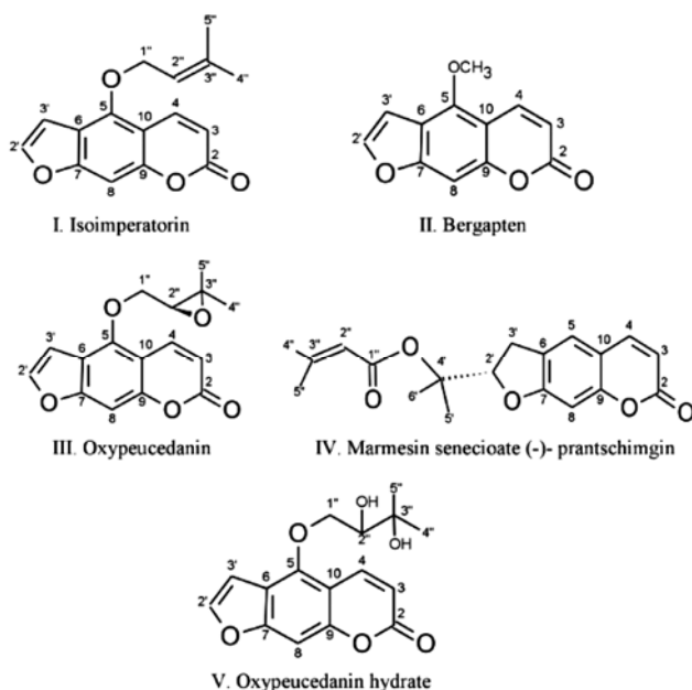
Fig. 1 — Structures of compounds I-V
