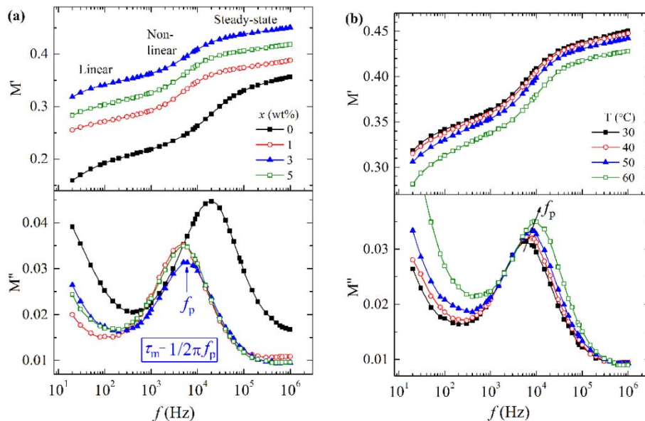
Fig. 4 — Frequency dependent real part M' and loss part M'' of complex electric modulus of (a) (PVA-PEO)/ x wt% \text{SnO}_2 films ( x = 0, 1, 3, and 5 ) at 30 °C, and (b) (PVA-PEO)/3 wt% \text{SnO}_2 film at different temperatures.
