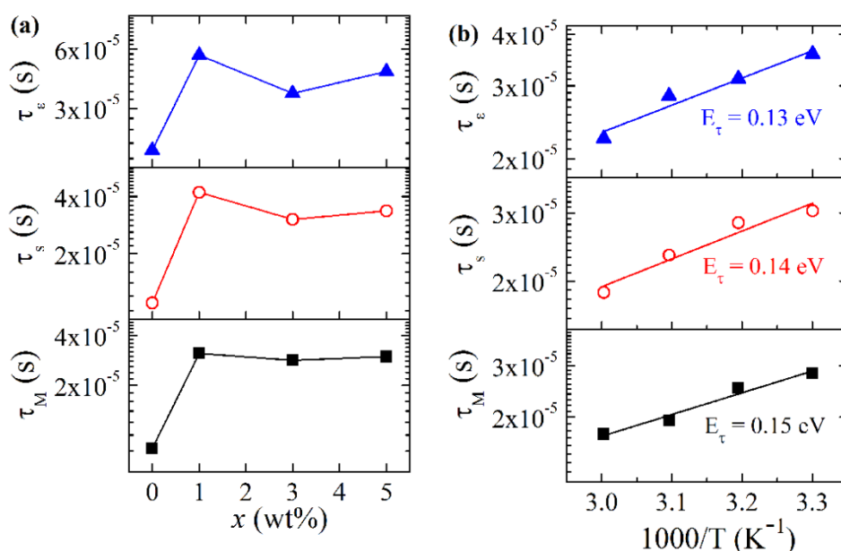
Fig. 5 — (a) SnO 2 concentration dependent relaxation times \tau_\epsilon , \tau_s and \tau_M of (PVA-PEO)/ x wt% SnO 2 films ( x = 0, 1, 3, and 5 ) at 30 °C and (b) Arrhenius behaviour of relaxation times of (PVA-PEO)/3 wt% SnO 2 film.
