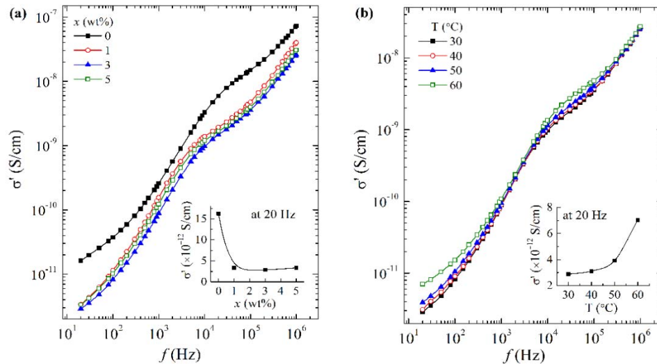
Fig. 6 — Frequency dependent real part \sigma' of (a) (PVA-PEO)/ x wt% SnO 2 films ( x = 0, 1, 3, and 5 ) at 30 °C, and (b) (PVA-PEO)/ 3 wt% SnO 2 film at different temperatures. The insets present \sigma' values at 20 Hz versus varying SnO 2 concentrations x (wt%) and different temperatures
