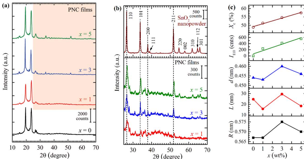
Fig. 1 — XRD patterns of (a) (PVA-PEO)/ x wt% SnO 2 films ( x = 0, 1, 3, \text{ and } 5 ), (b) the SnO 2 nanopowder and the enlarged view of SnO 2 peaks in PNC films, and (c) the plots of X_c , I_{110} , d , L , and R versus varying SnO 2 concentrations x (wt%) of the PNC films.
