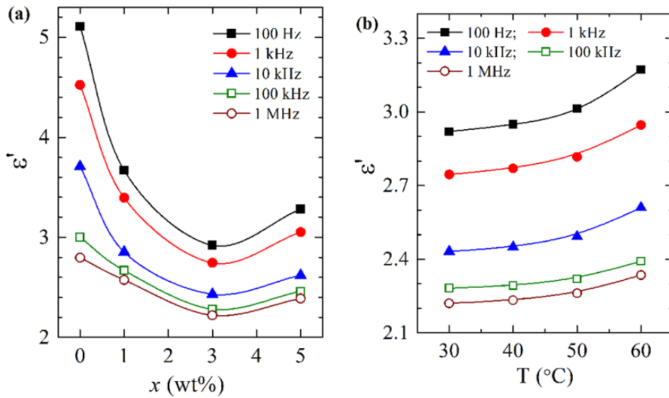
Fig. 3 — (a) \text{SnO}_2 concentration dependent values of \epsilon' for (PVA-PEO)/ x wt% \text{SnO}_2 films ( x = 0, 1, 3, and 5 ) at 30 °C and (b) temperature dependent \epsilon' values of (PVA-PEO)/3 wt% \text{SnO}_2 film at various frequencies.
