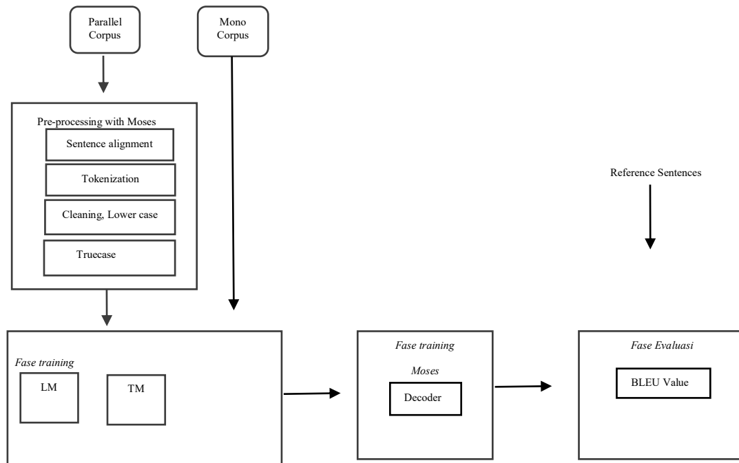
Figure 2. ARCHITECTURE IN SMT BUILDING
