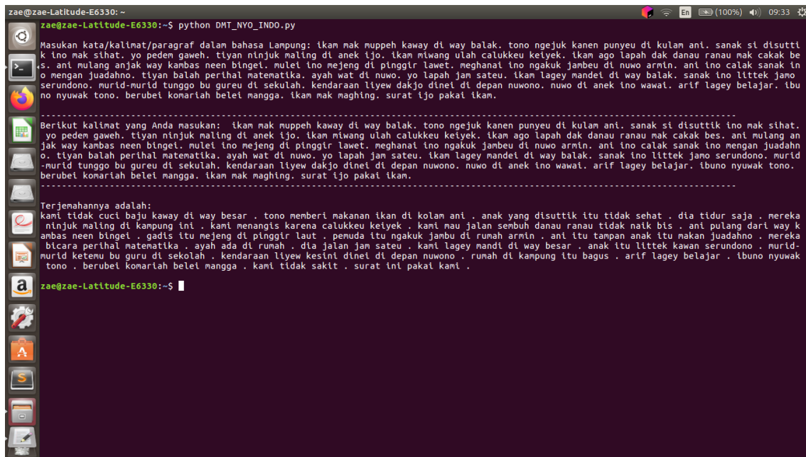
Figure 3. RESULTS OF PURWARUPA TRANSLATING LAMPUNG WITH NYO DIALECT
